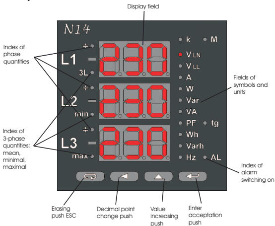
Fig. 4 Frontal panel
