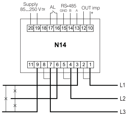
Direct measurement in a 3-wire network
