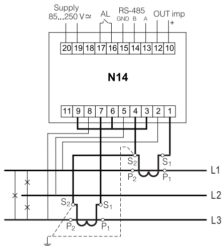
Semi-indirect measurement in a 3-wire network
