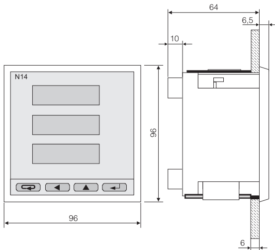
Fig. 1. Overall meter dimensions
