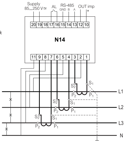
Semi-indirect measurement in a 4-wire network
