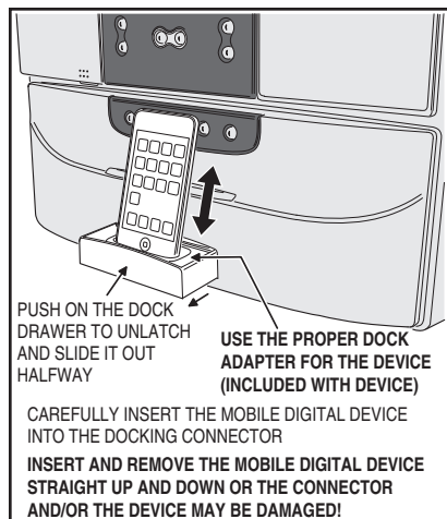
Figure 19. Device in Dock
