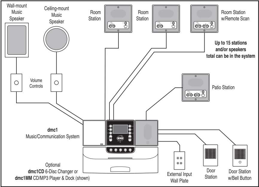
Figure 1. System Overview
