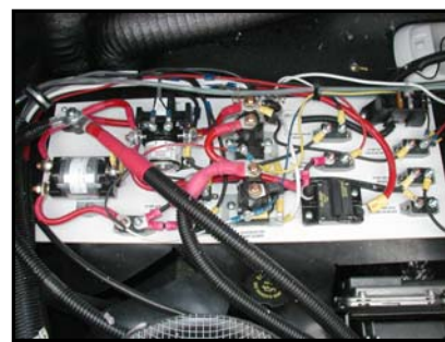
Figure 7-11. Circuit Breakers
