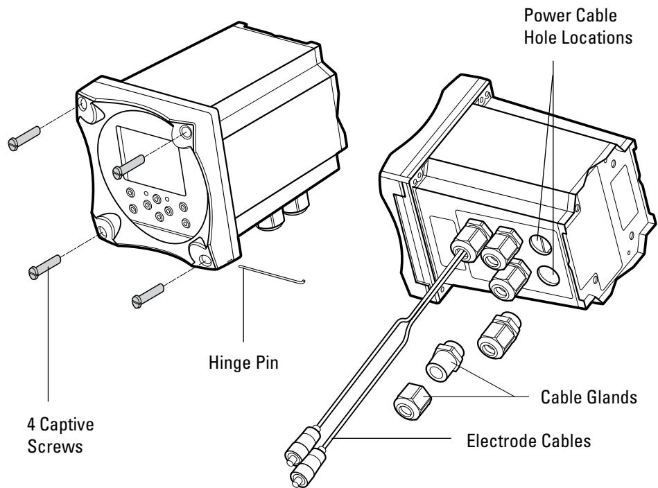
Figure 2-4 —Electronics Enclosure with Cable Glands
