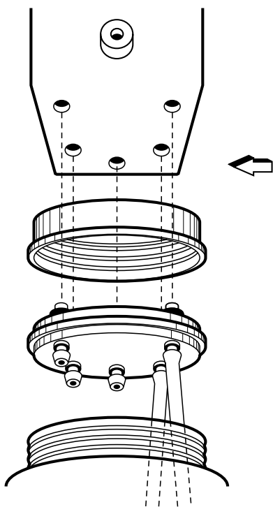
Figure 5-1 – Reagent Bottle Assembly
