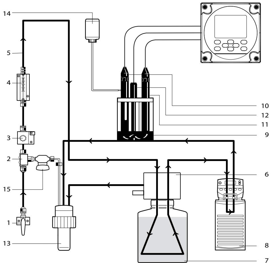
Figure 1-2 —Flow During Normal Operation
