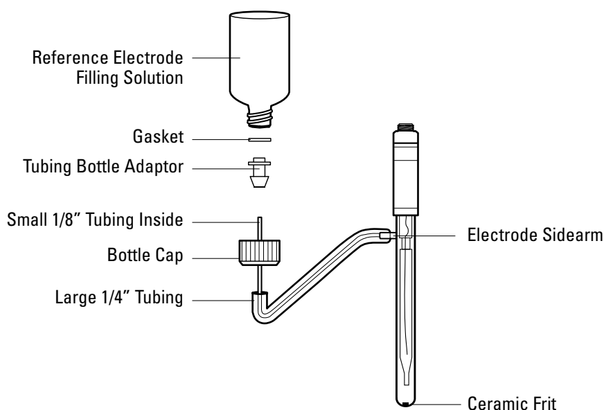
Figure 2-9 —Reference Electrode with Filling Solution
