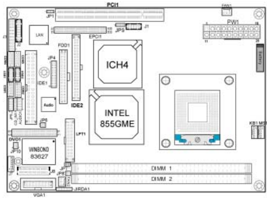
EBC-I855C Connector, Jumper and Component locations
