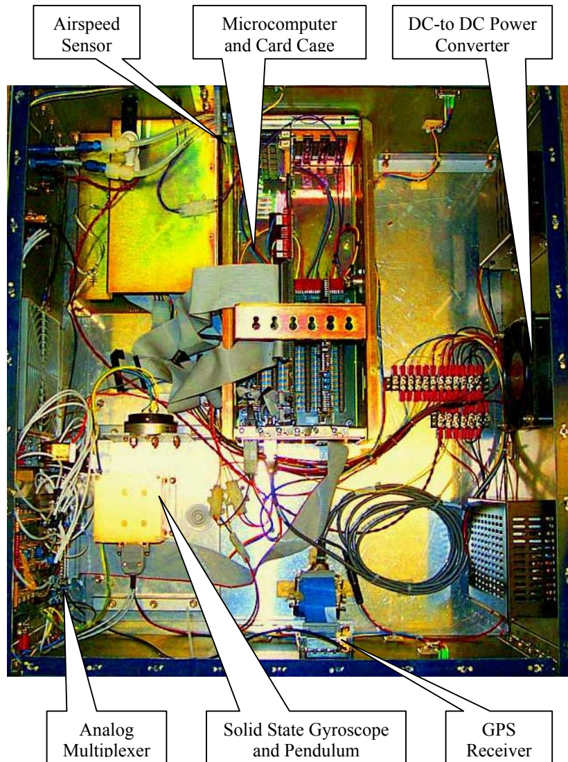
Figure 1: Component Layout
