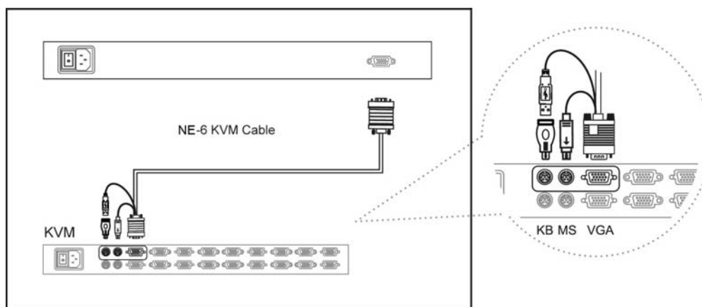
Figure 7. Example of connecting NE-6 4-in-1 Combo KVM cable to KVM via PS/2 interface
