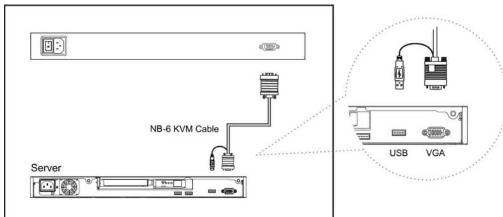
Figure 4 Example of connecting NB-6 2-in-1 USB KVM cable to server via USB interface
