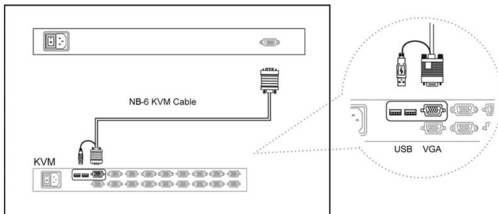
Figure 5 Example of connecting NB-6 2-in-1 USB KVM cable to KVM via USB interface
