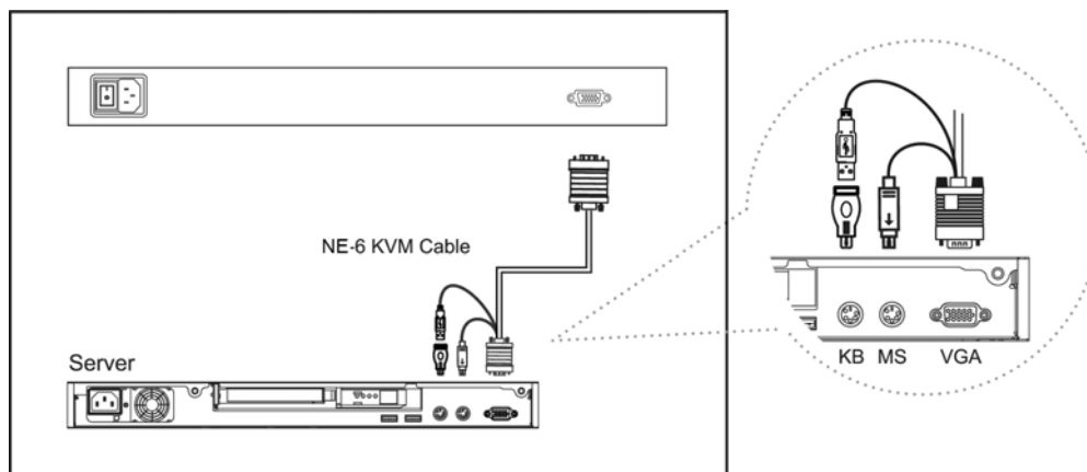
Figure 6. Example of connecting NE-6 4-in-1 Combo KVM cable to server via PS/2 interface
