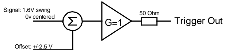
Trigger Output Block diagram:
