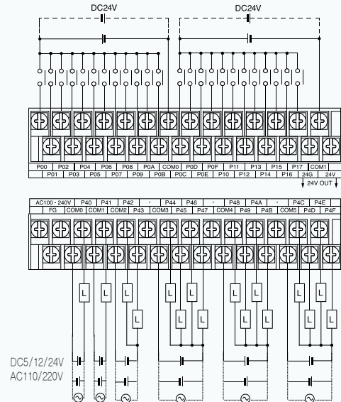
● K7M-DR40U
