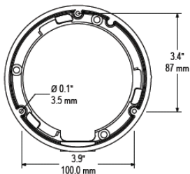
Base hole positions
