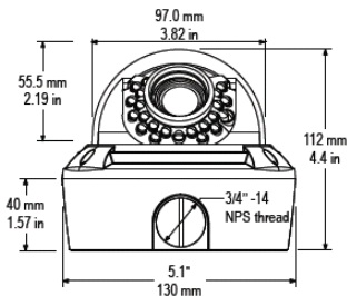
Vandal Dome Dimensions
