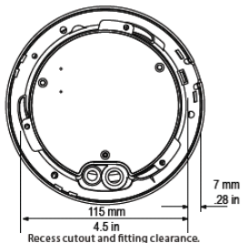
Recess cutout and fitting clearance.
