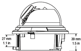
Indoor Dome Dimensions
