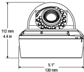
Indoor Dome Dimensions
