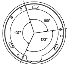
Underside Base hole positions
