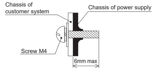
Fig.5.7 Mounting screw
