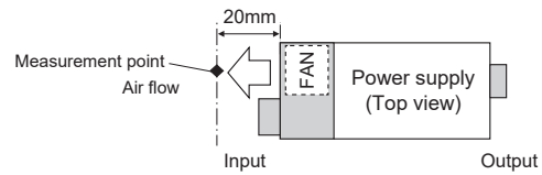
Fig.5.6 Measurement of FAN exhaust temperature
