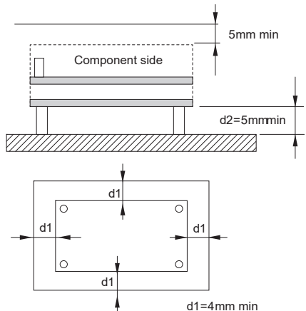
Fig.3.13 Installation method
