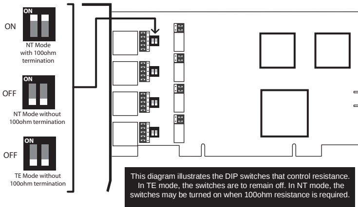
Figure 4: NT Termination Switches
