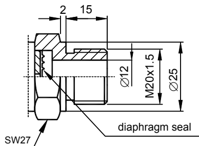
Fig.3. M-type pressure connector with M20x1.5 thread
