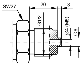
Fig.5. 1/2" NPT type and G1/2" type pressure connector with G1/2" thread
