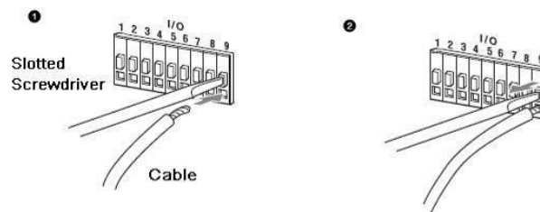
Figure 3-16 I/O port
