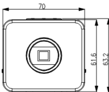
Figure 2-3 Front panel
