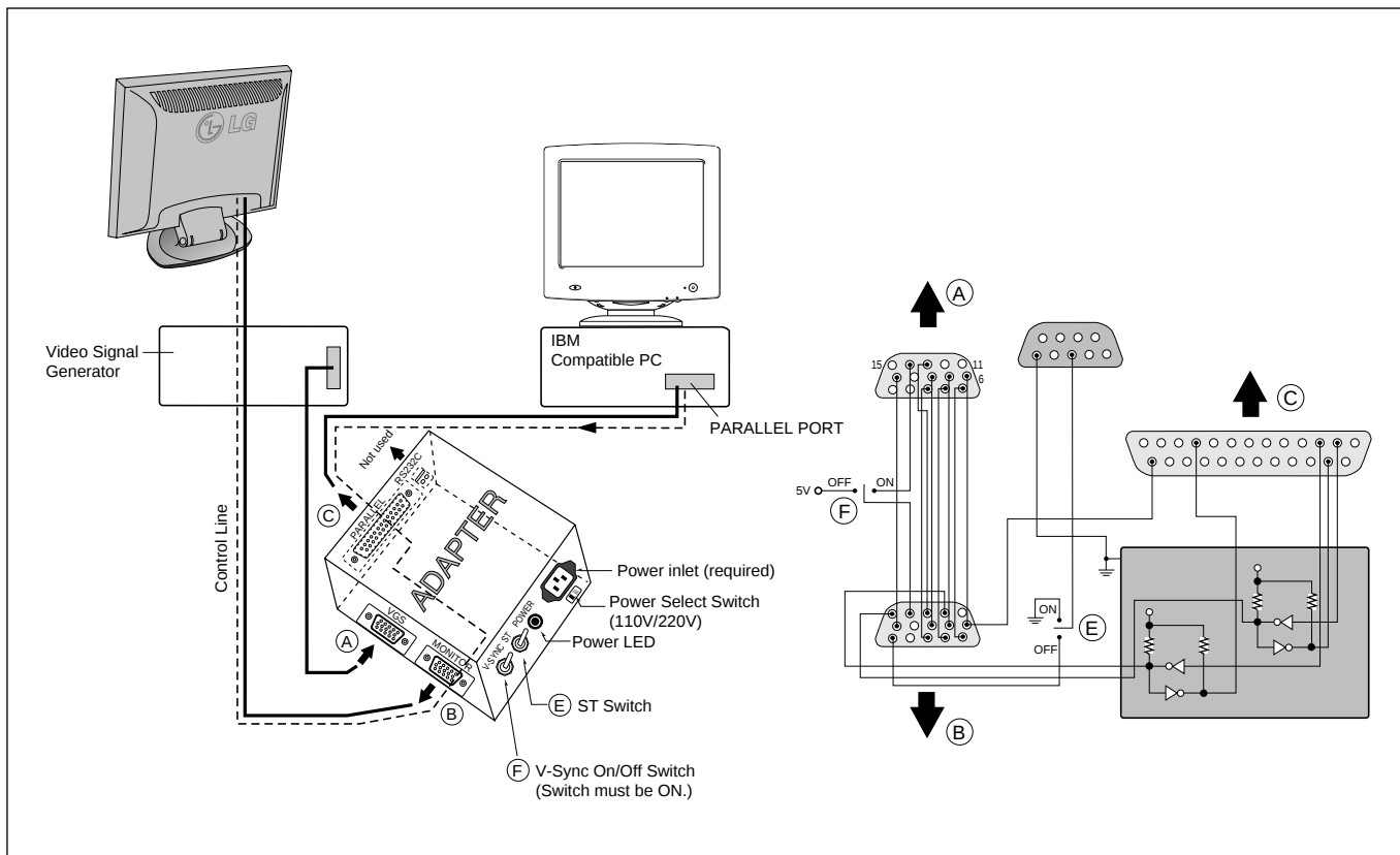
Figure 1. Cable Connection
