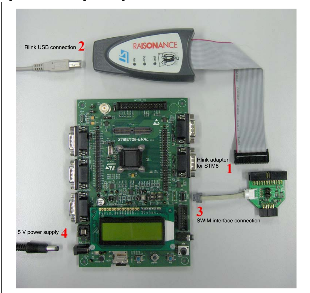
Figure 25. Connecting the debug instrument to the STM8 evaluation board
