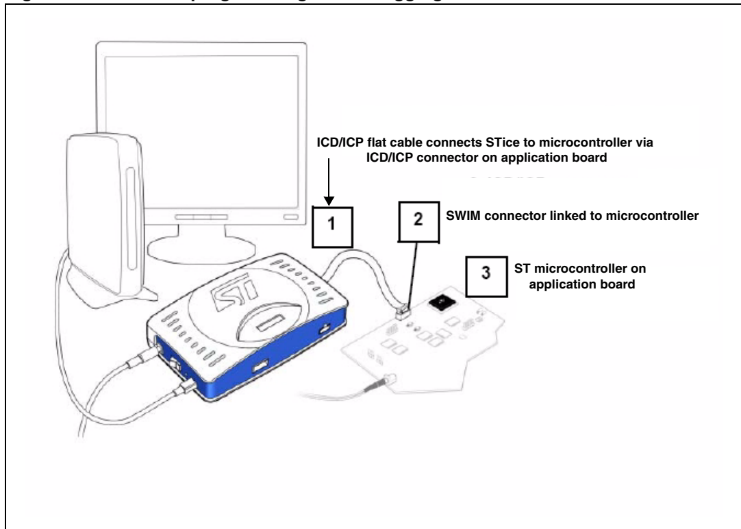
Figure 17. In-circuit programming and debugging
