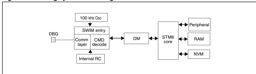
Figure 13. Debug system block diagram
