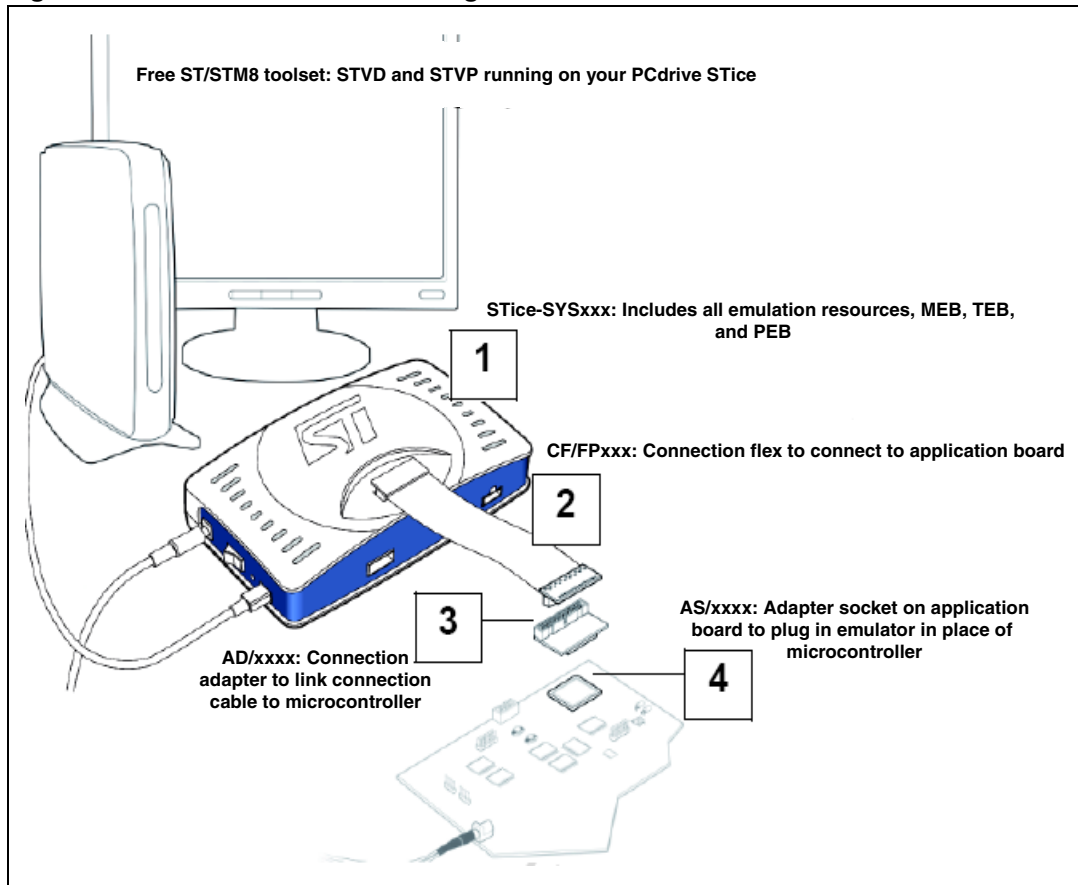
Figure 16. STice in emulation configuration
