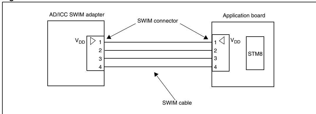
Figure 14. Hardware connection
