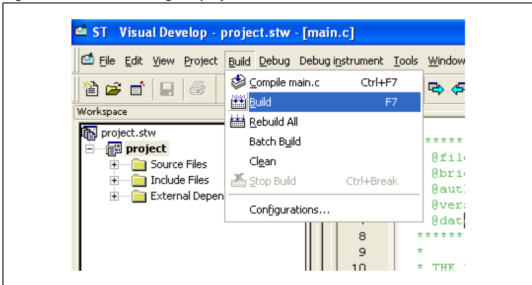
Figure 23. STVD: Building the project
