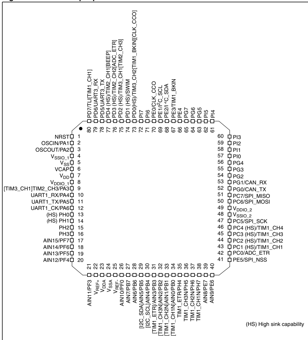
Figure 12. LQFP 80-pin pinout
