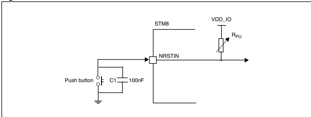
Figure 10. RC circuit
