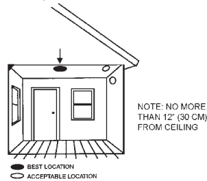
Figure 5: RECOMMENDED SMOKE ALARM MOUNTING LOCATION
