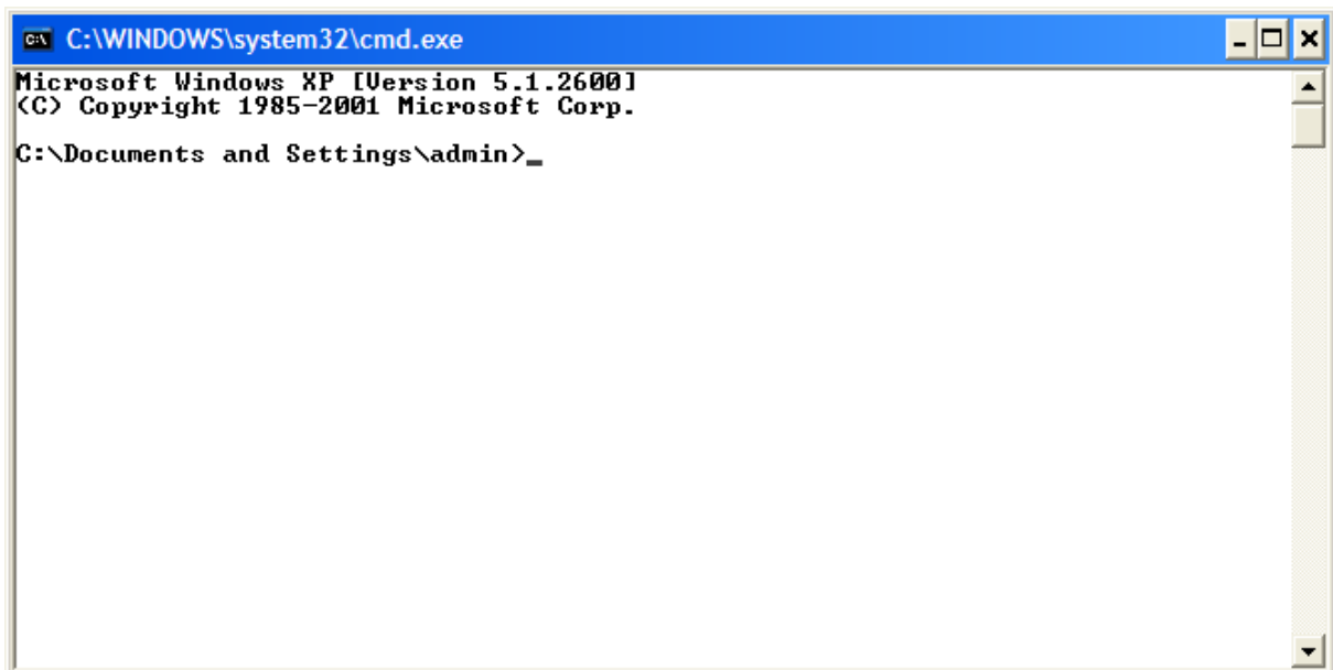
Figure 2.6: DOS prompt.
