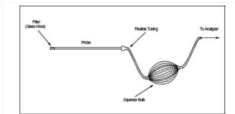
Figure 3-2. Integrated Gas-Sampling Train.
