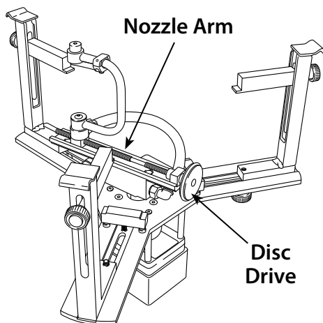
Complete Assembly
