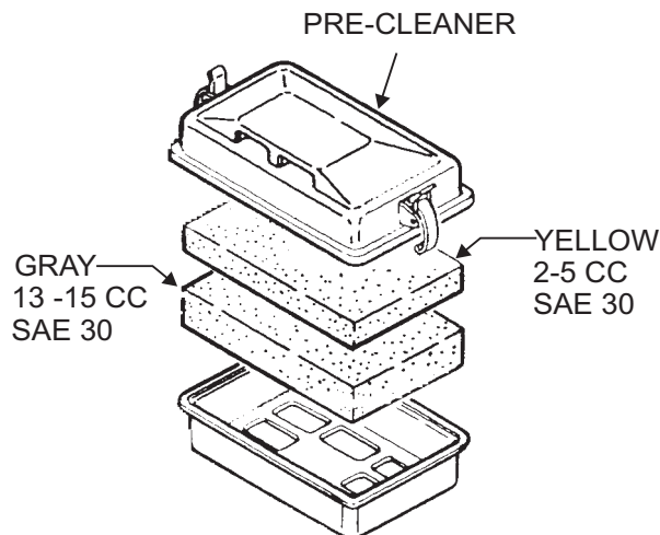
Figure 13. Pre-Cleaner
