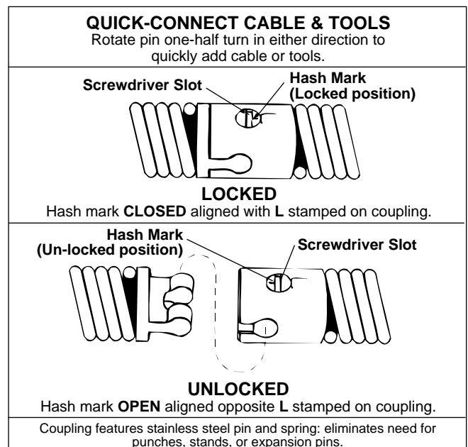
Figure 3 – Disconnecting/Connecting Cable to Pigtail or Tool
