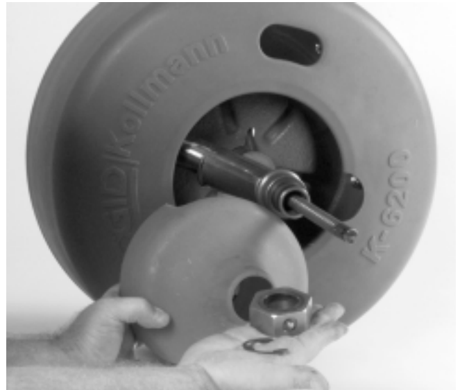
Figure 13 – Remove Retaining Ring and Inner Drum
