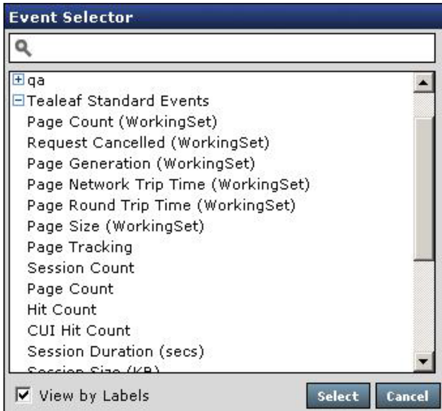
Figure 5. Event Selector
