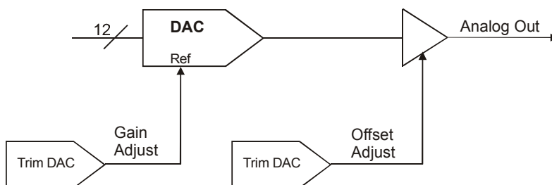
Figure 5-2. Analog output calibration – elements
