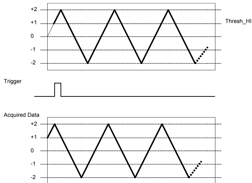
Figure 4-15. Trigger Positive Slope
