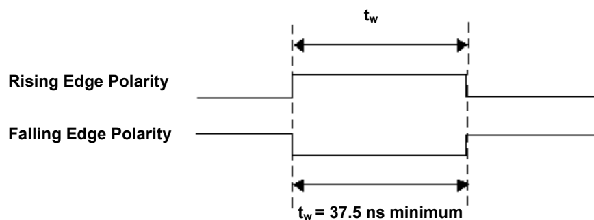
Figure 4-25. D/A CONVERT input signal timing
