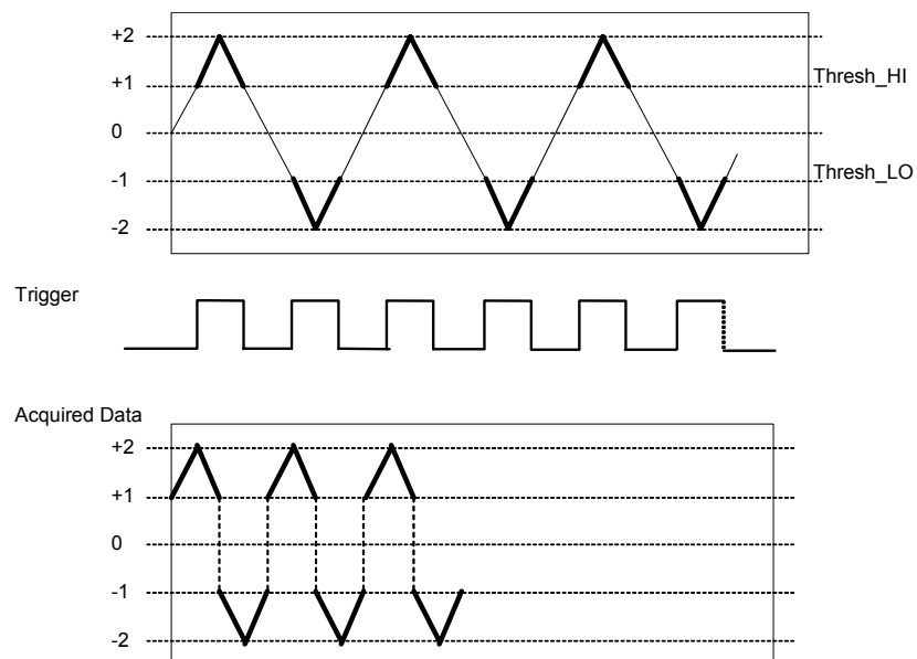
Figure 4-22. Gate Outside Window
