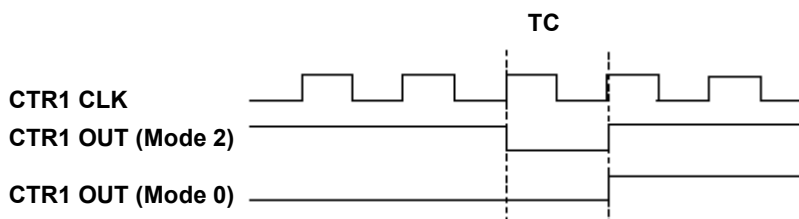
Figure 4-30. CTR1 OUT signal timing
