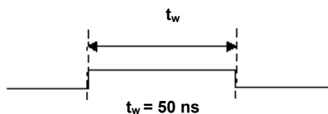
Figure 4-14. A/D STOP Signal Timing
