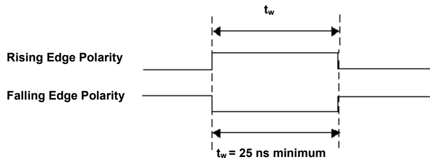
Figure 4-29. CTR1 GATE signal timing
