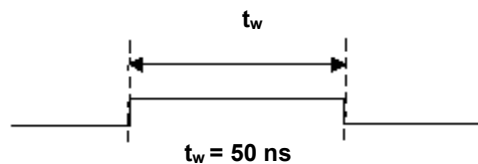
Figure 4-24. D/A START TRIGGER output signal timing
