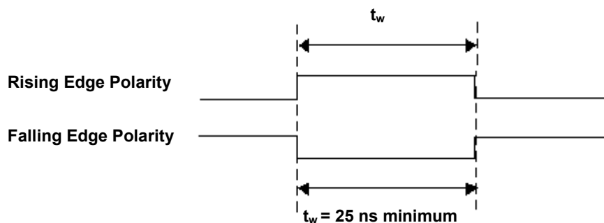
Figure 4-32. CTR2 GATE signal timing
