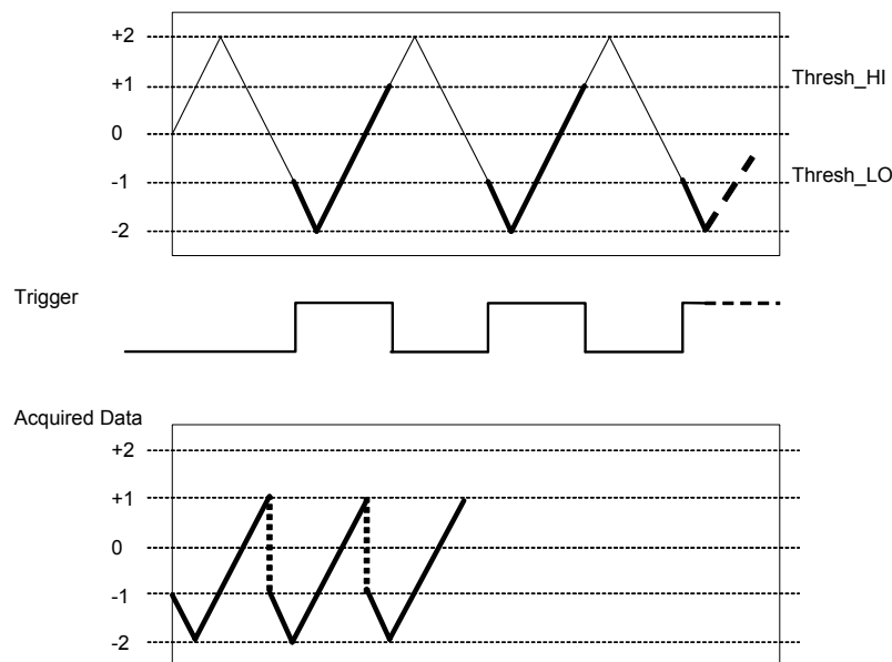
Figure 4-20. Gate Positive Hysteresis
