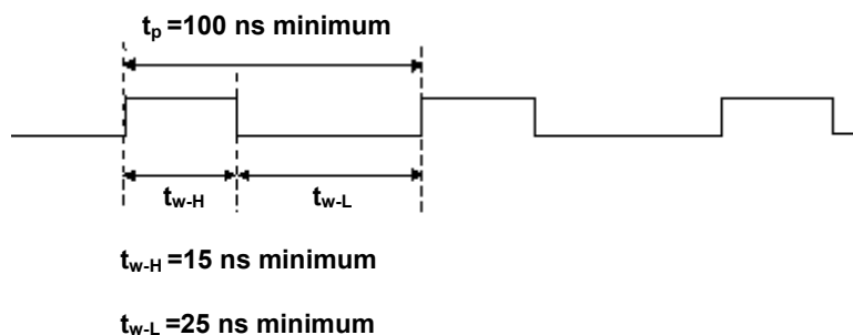
Figure 4-28. CTR1 CLK signal timing
