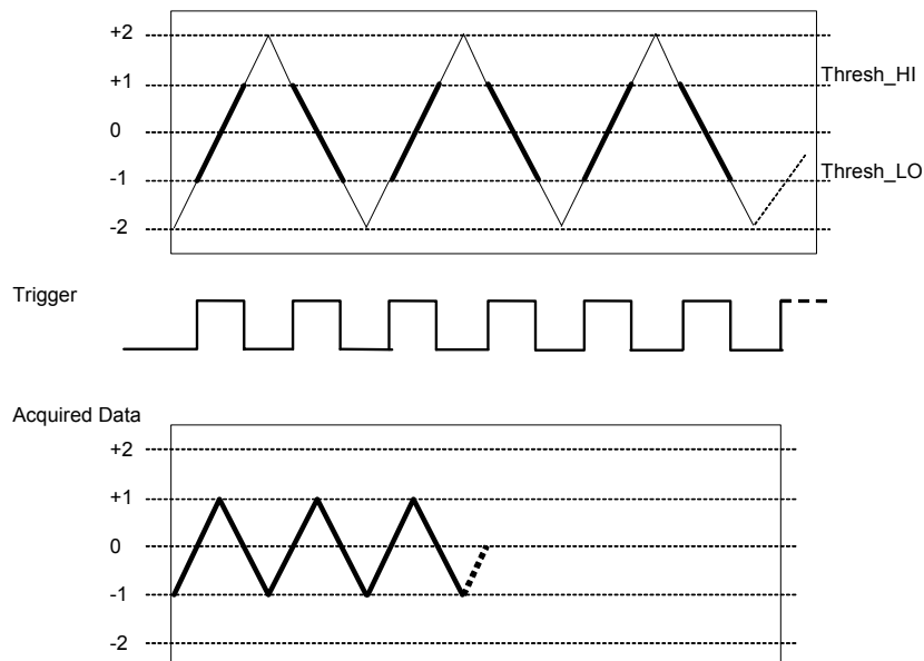
Figure 4-21. Gate Inside Window
