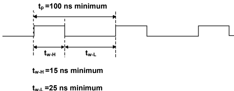
Figure 4-31. CTR2 CLK signal timing
