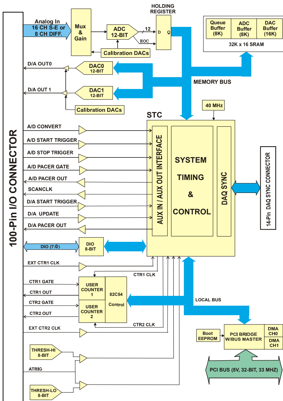
Figure 4-1. Block diagram – PCI-DAS6070
