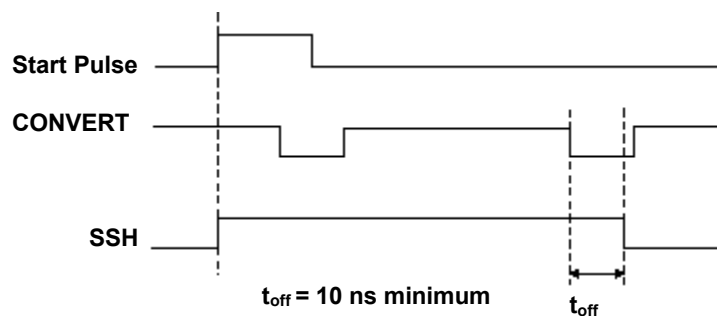
Figure 4-10. SSH Signal Timing
