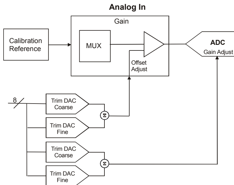
Figure 5-1. Analog input calibration - basic elements
