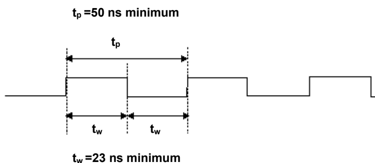
Figure 4-27. D/A EXTERNAL TIME BASE signal timing
