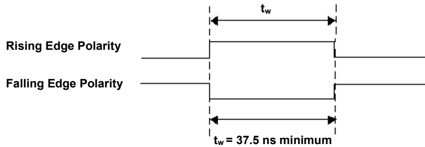
Figure 4-4. A/D START TRIGGER input signal timing
