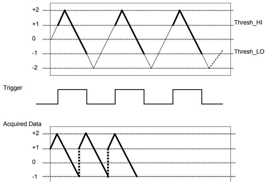
Figure 4-19. Gate Negative Hysteresis
