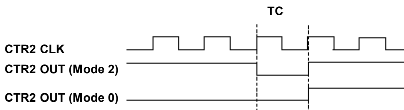
Figure 4-33. CTR2 OUT signal timing
