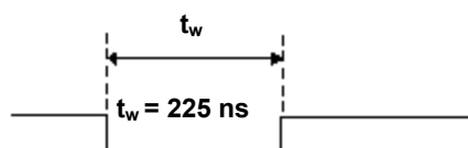
Figure 4-26. D/A CONVERT output signal timing
