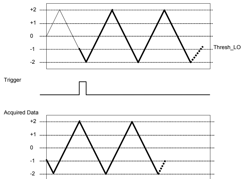
Figure 4-16. Trigger Negative Slope
