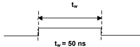
Figure 4-5. A/D START TRIGGER output signal timing
