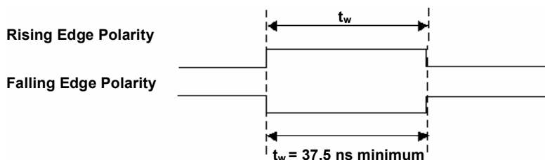
Figure 4-11. A/D CONVERT signal input timing requirement
