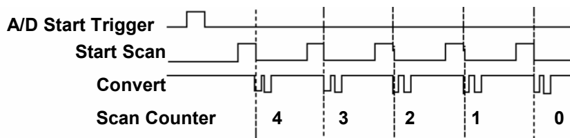
Figure 4-3. Data Acquisition example for conventional triggering
