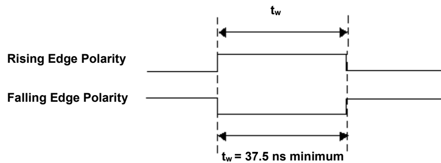
Figure 4-23. D/A START TRIGGER input signal timing
