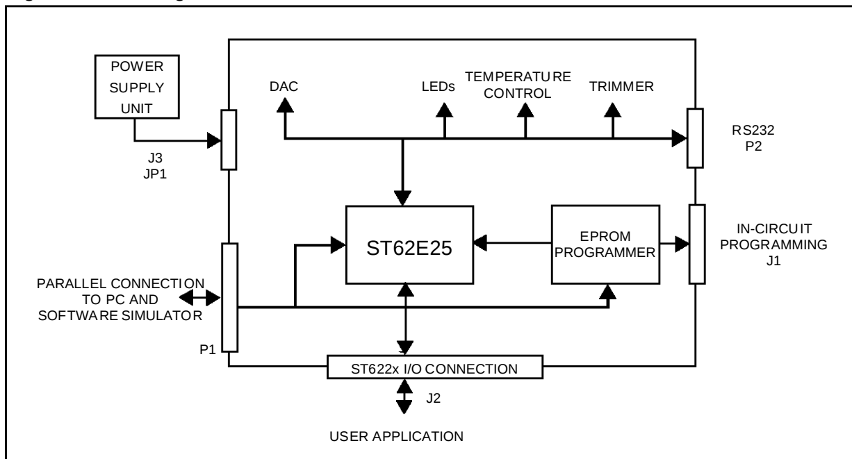
Figure 1. Block Diagram of ST622x Starter Kit
