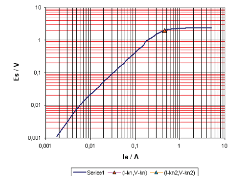
Excitation curve down to 1 mV
