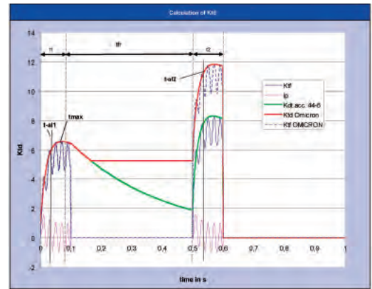
Automated calculation of K_{td} without remanence according to IEC 60044-6 and with remanence ( K_{td} OMICRON)
