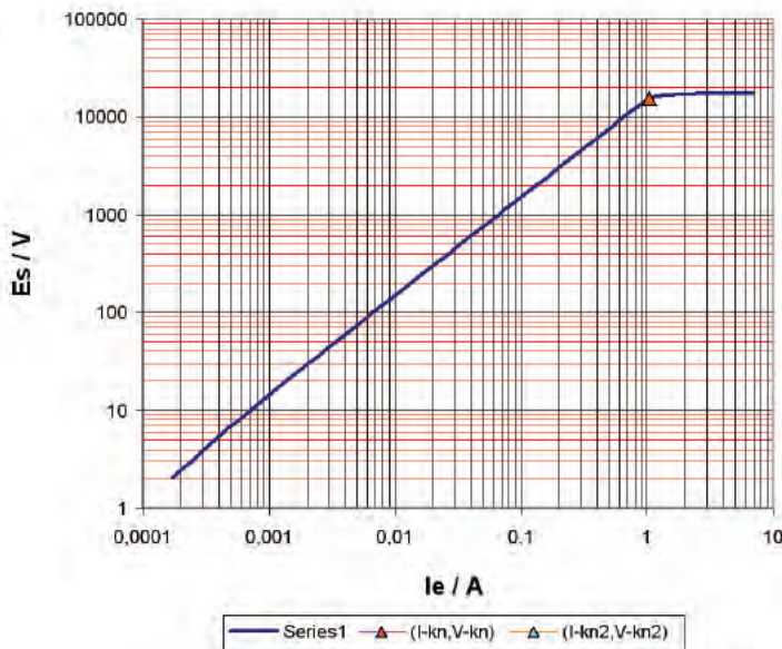
Excitation test example for 17 kV
