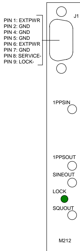
Figure C-1, M212 Front Panel I/O Signals
