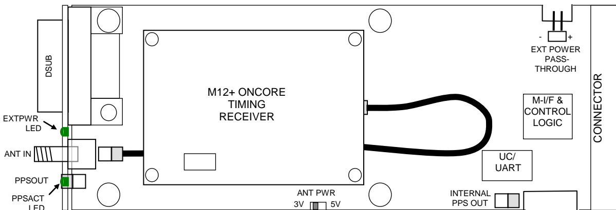
Figure 3-2, M213 Physical Layout
