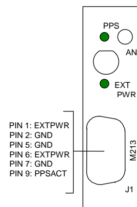
Figure 3-3, M213 Front Panel
