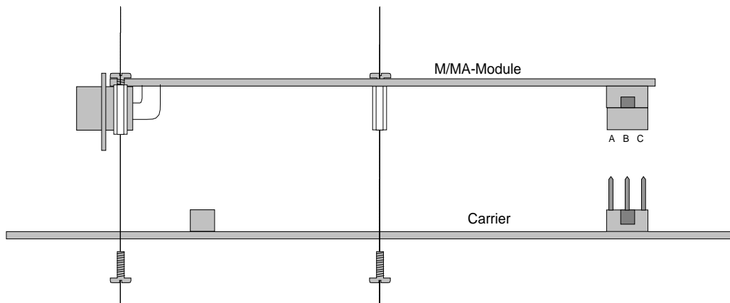
Figure 4-1, M-MODULE Installation
