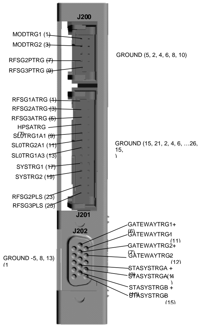
Figure F-1, M1721 Front Panel Connectors
