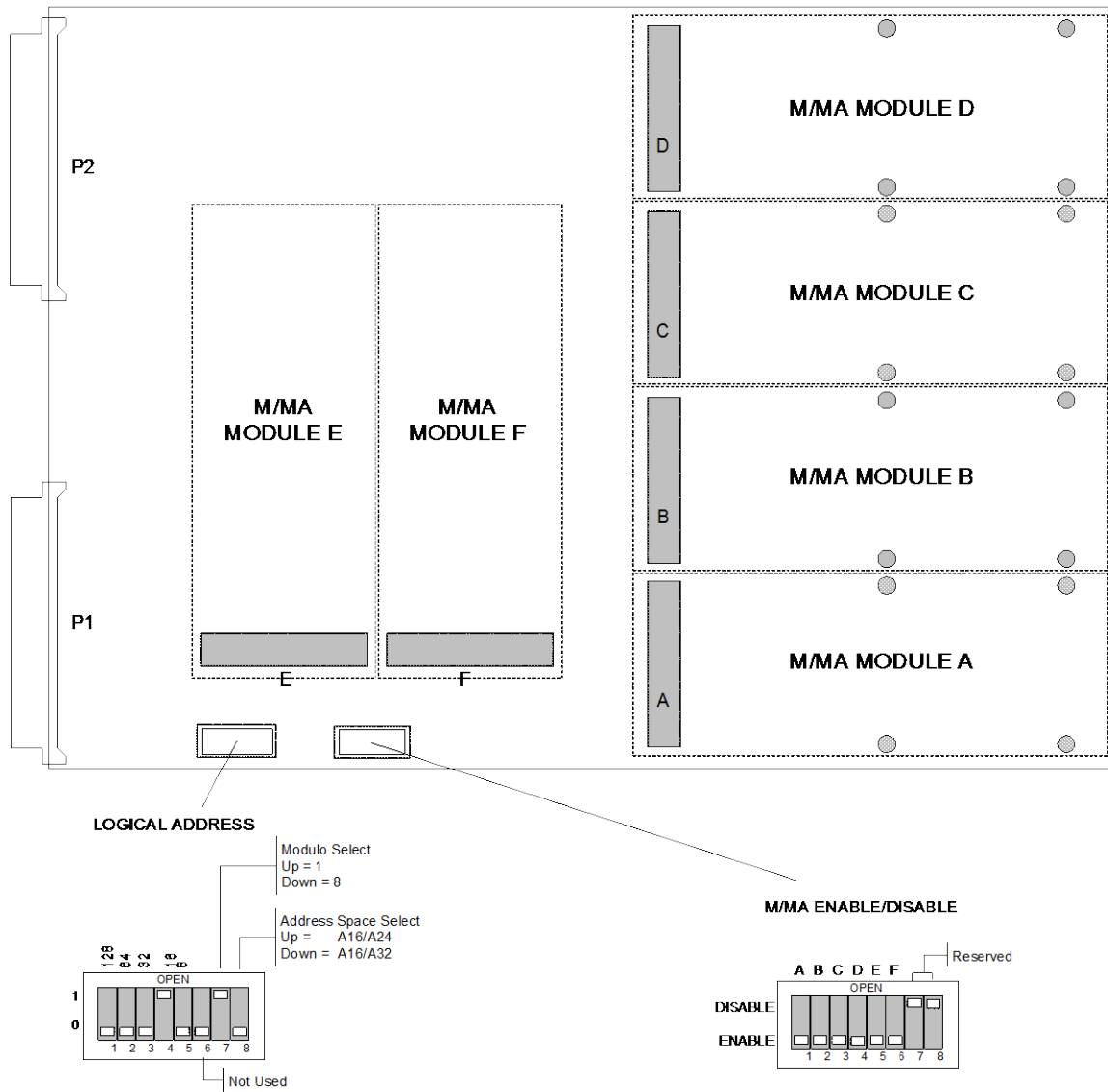
Figure 2-4, VX405C Hardware Configurable Controls
