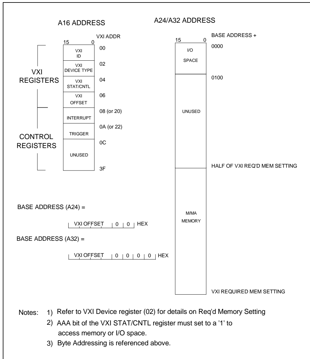
Figure 2-3, Memory Organization
