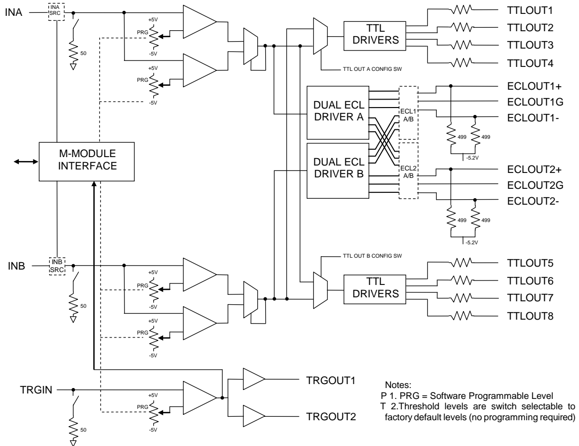
Figure 6-1, Functional Block Diagram
