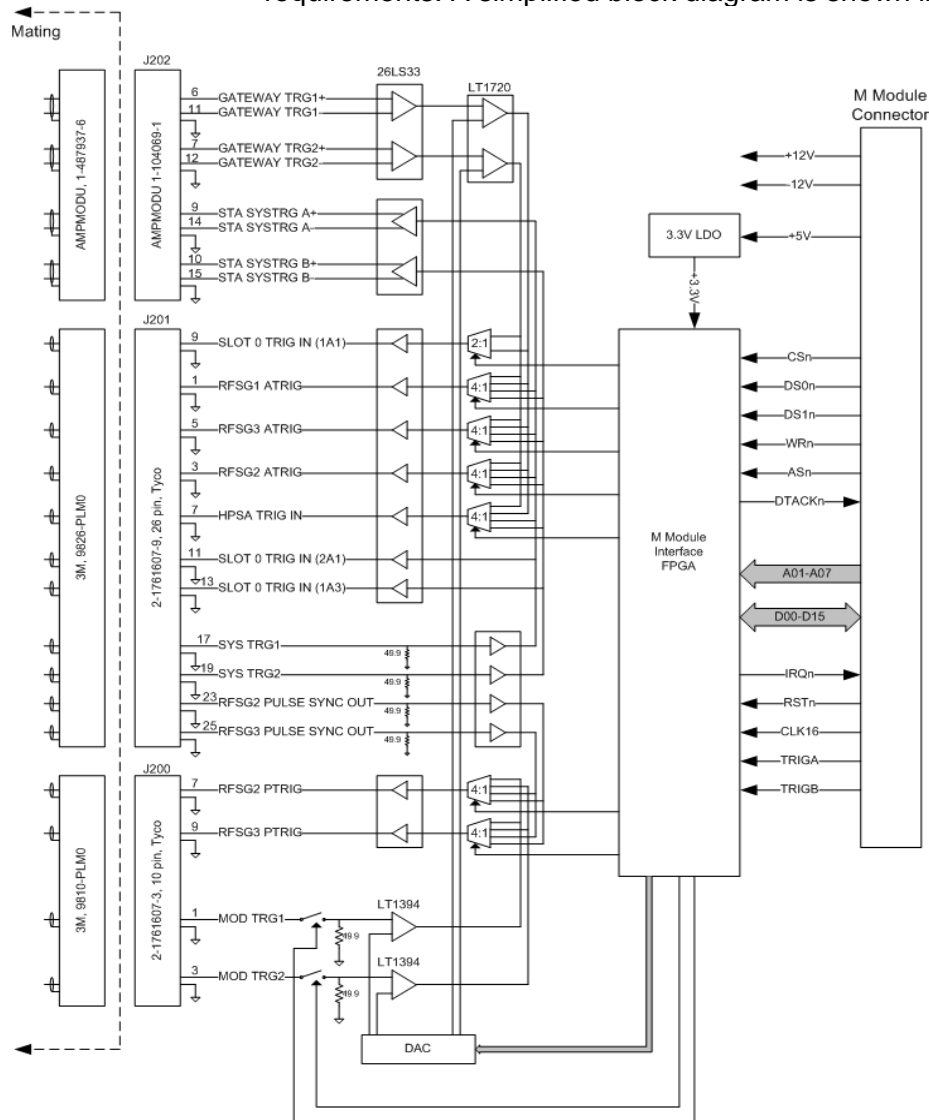
Figure 8-1, Functional Block Diagram
