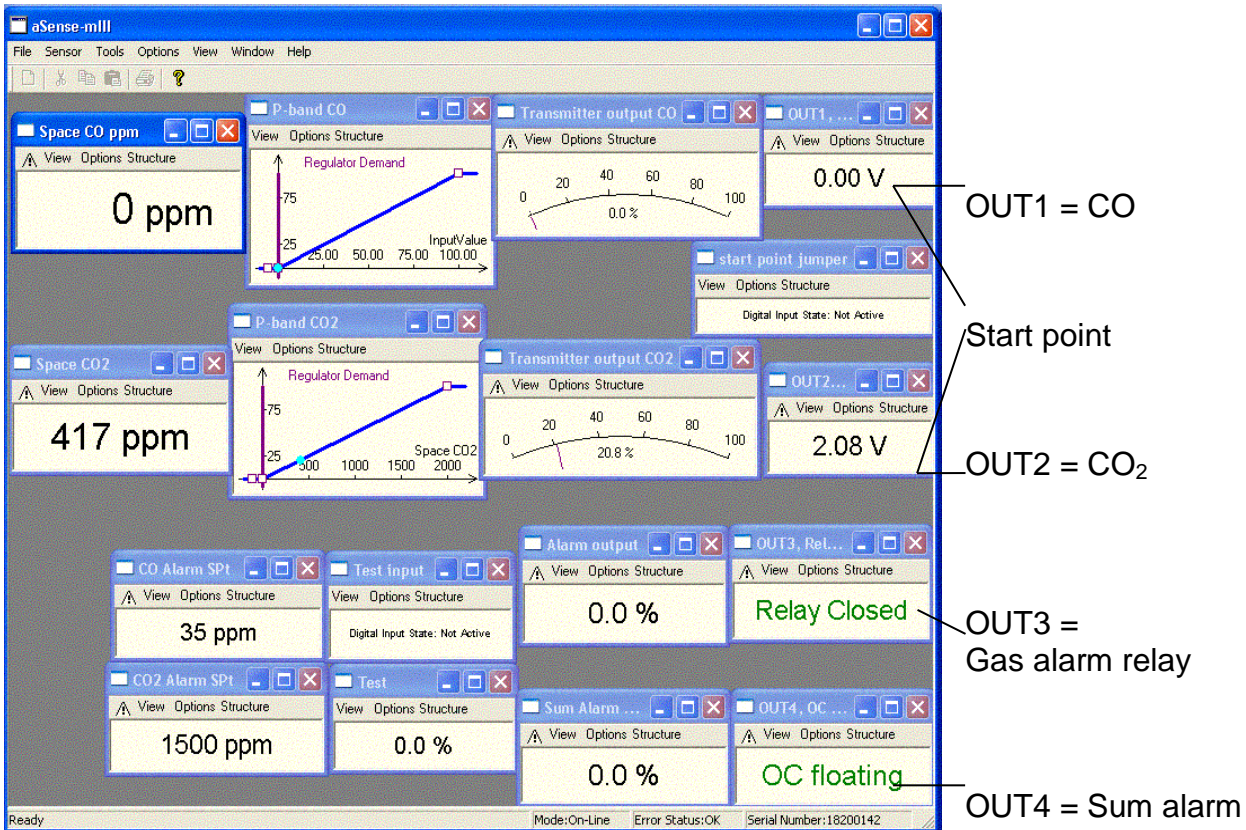
Figure 2 Print screen of UIP4.3 PC work space of a SENSE mIII where the pre-set functions can easily be redefined. The four outputs (far right) are here arranged in rows together with the function blocks that control the output.
