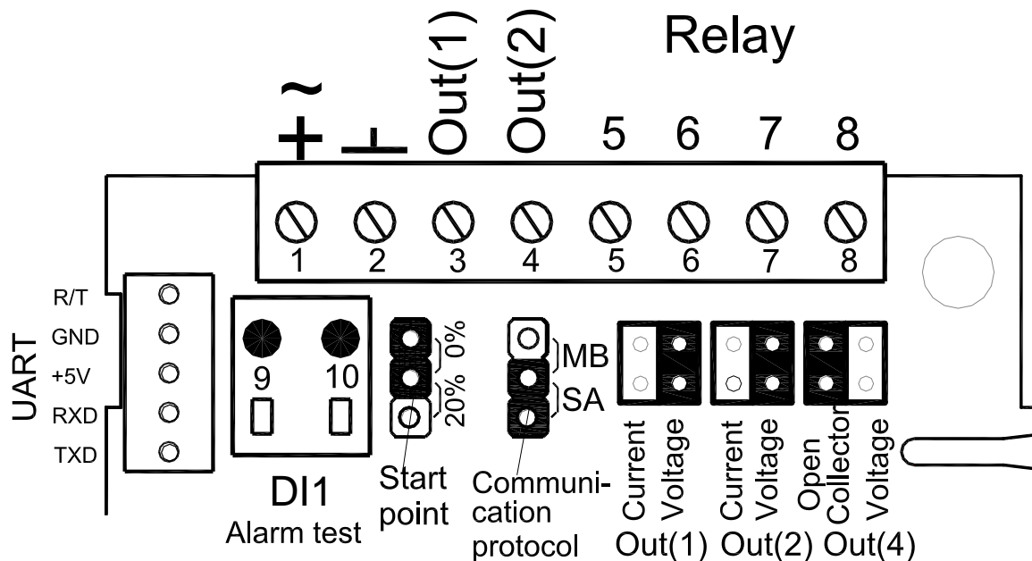
Figure 12. The aSENSE mIII printed circuit board with the connection terminal area is enlarged. The terminal DI1 may be used for forced ventilation. If the sensor has a heater it is connected to \sim and \pm .
