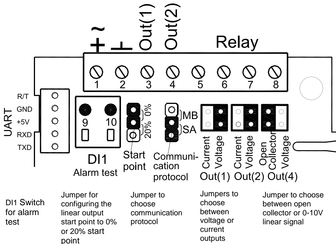
Figure 5 The connection terminal area of the aSENSE mIII with jumpers and terminals. The terminal
