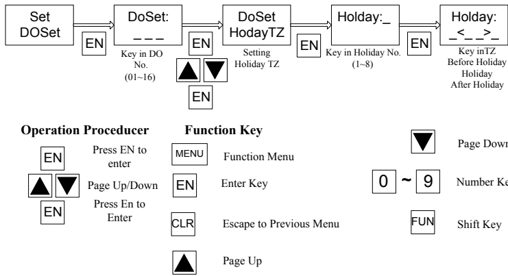
Figure 4.4.1 Set DO Holiday Time Zone
