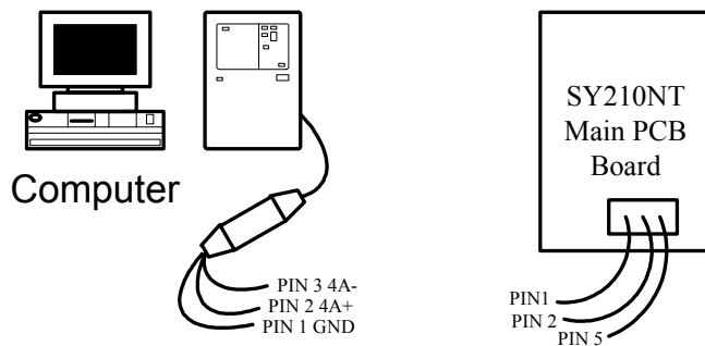
Figure 2.1 Connection from SY210NT to PC
