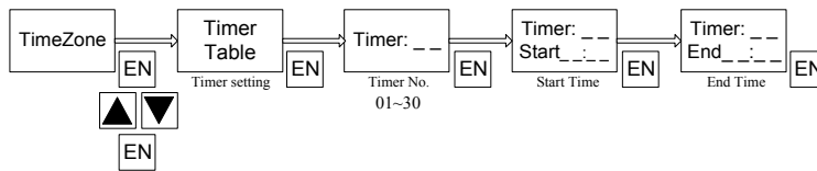
Figure 4.7.2 Set TimeZone
