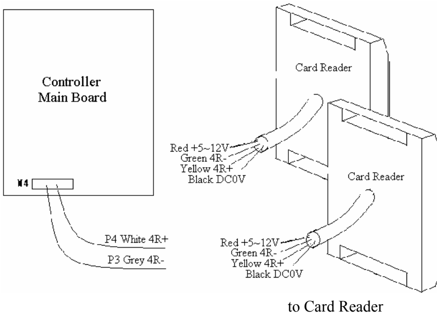
Fig 2.2 Connection from Controller to Card Reader
