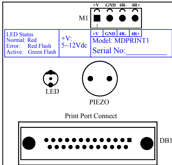
Figure 2.3.2 Connection of Printer Module
