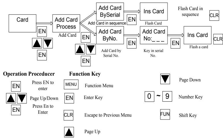
Figure 4.2.1 Store Card
