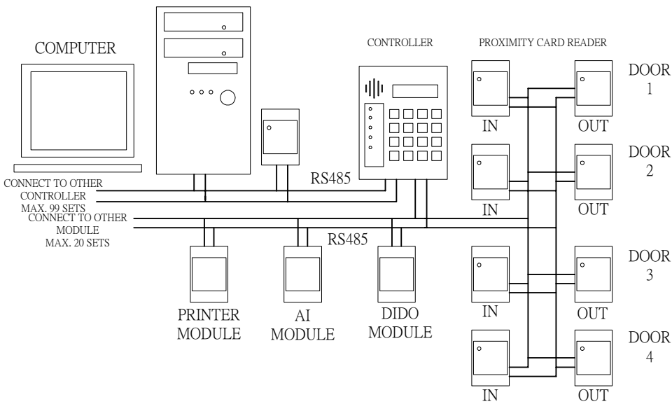
Figure 1.1 System Configuration
