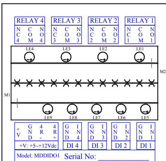
Figure 2.3.1 DI4Do4 Module Connection
