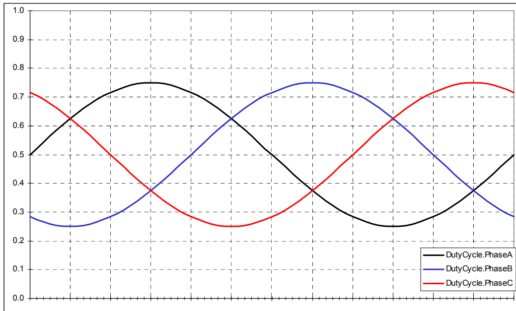
Figure 4-2. 3-Phase Sine Waves with Amplitude of 50%
