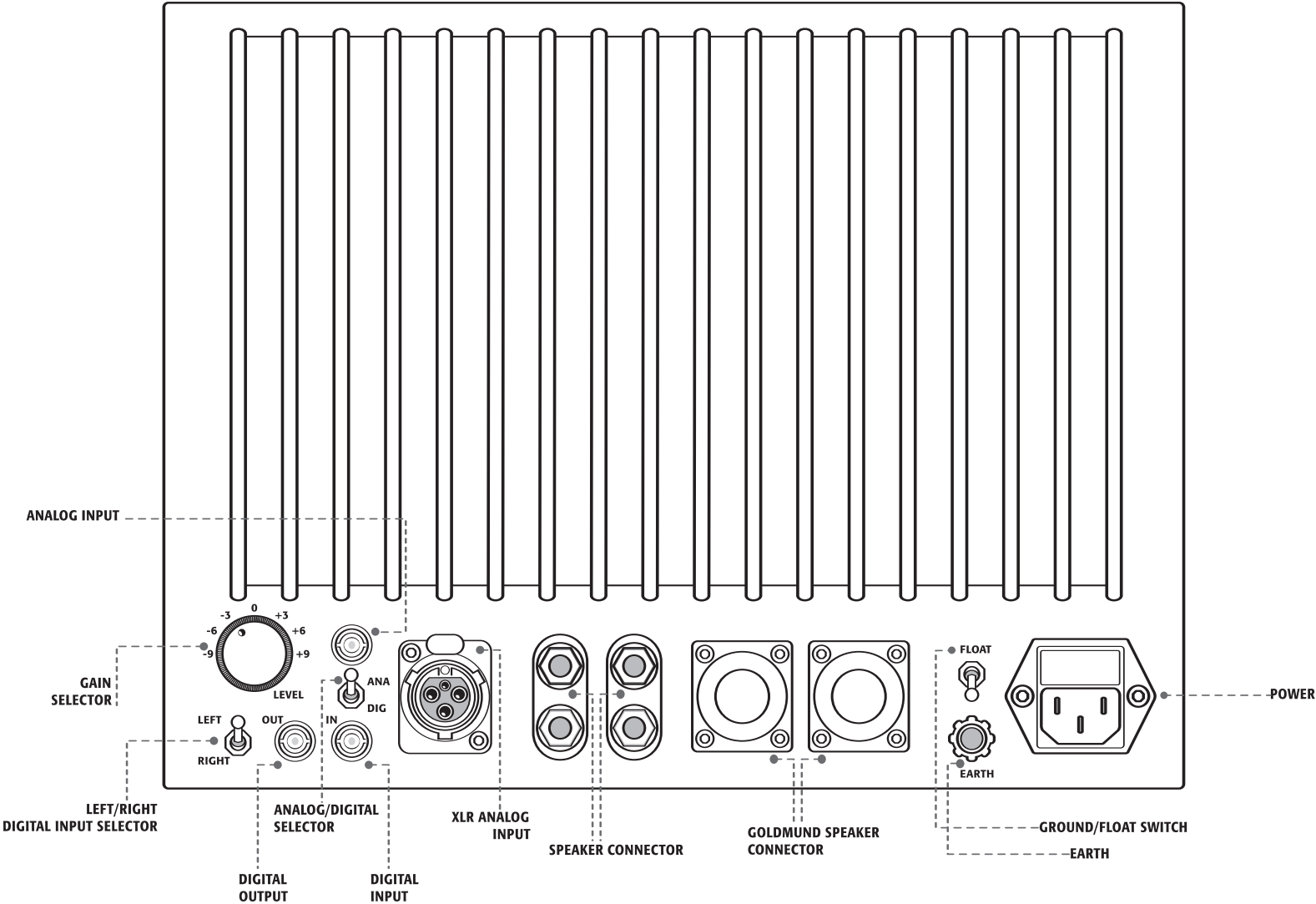
TELOS 600 Universal Power Amplifier | Back Panel
