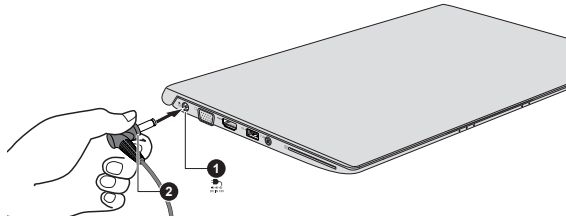
Figure 2-4 Connecting the DC output plug to the computer (Z40-B)
