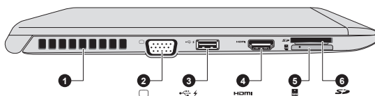
Figure 3-8 The left side of the computer (Z40-B)
