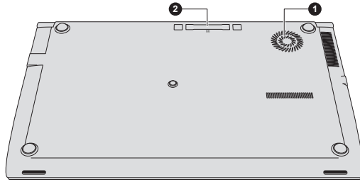
Figure 3-11 The underside of the computer (Z40-B)
