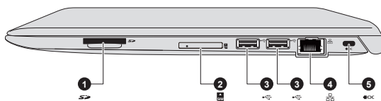
Figure 3-3 The right side of the computer (Z30-B)
