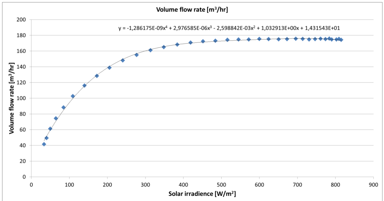
Figure 1- Volume flow rate
