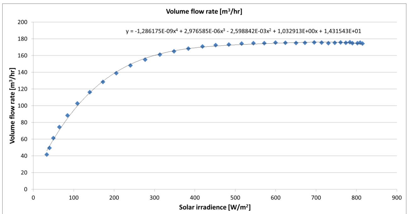
Figure 2 - Volume flow rate
