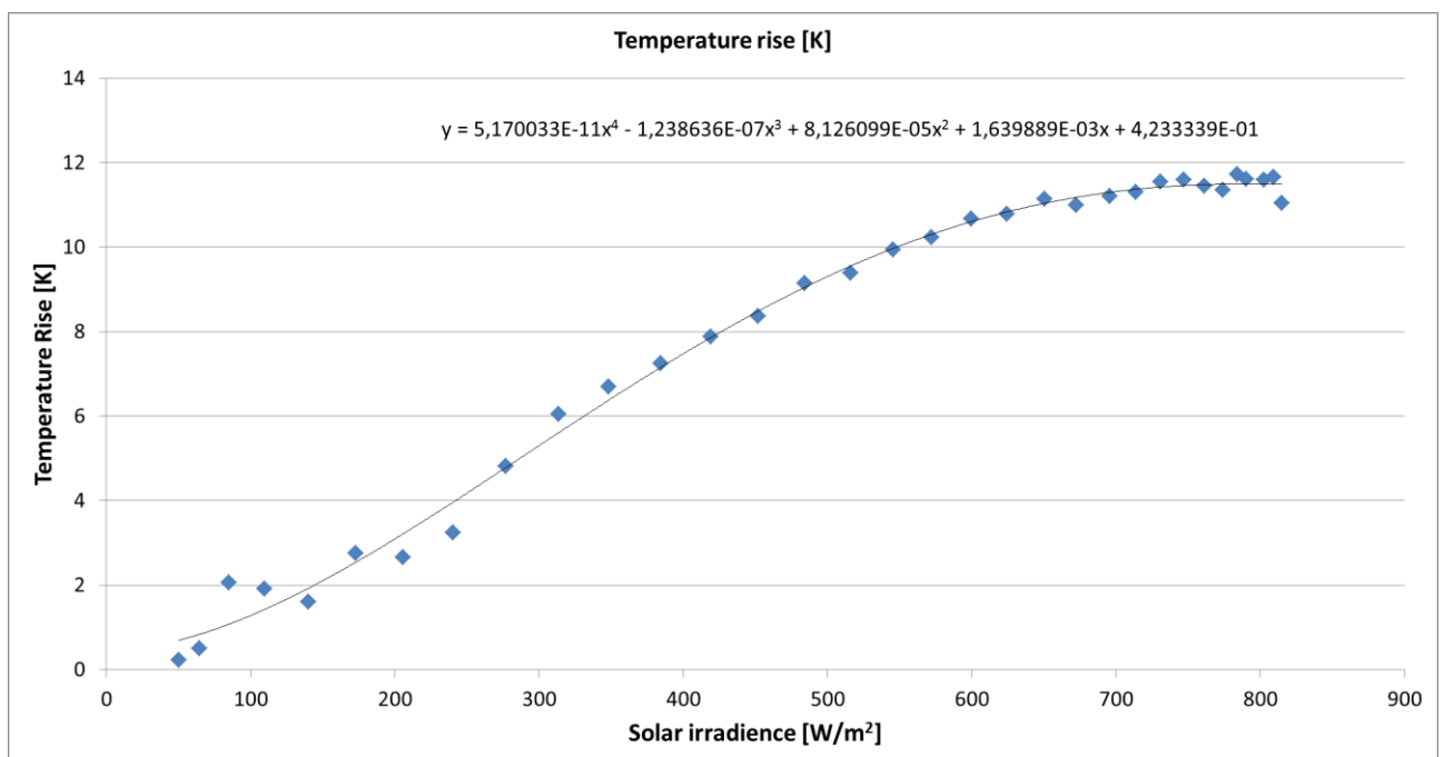
Figure 2 - Temperature rise
