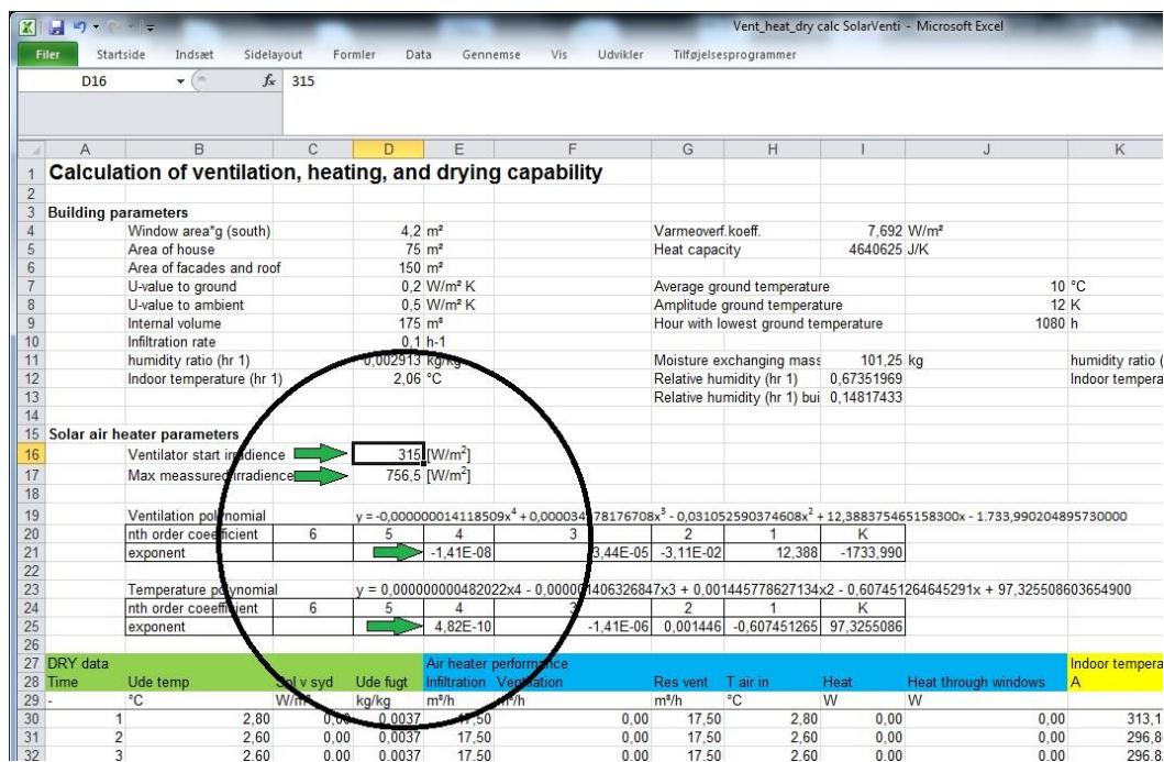
Figure 6 - Screenshot of the prepared calculation workbook for modeling/simulation of a solar air heater's performance parameters in a design reference year. Green arrows indicate input cells
