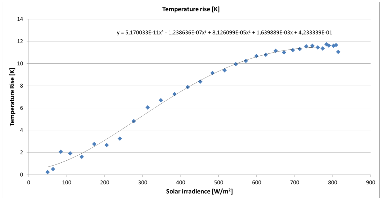
Figure 3 - Temperature rise
