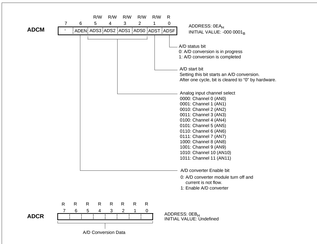
Figure 13-1 A/D Converter Control Register
