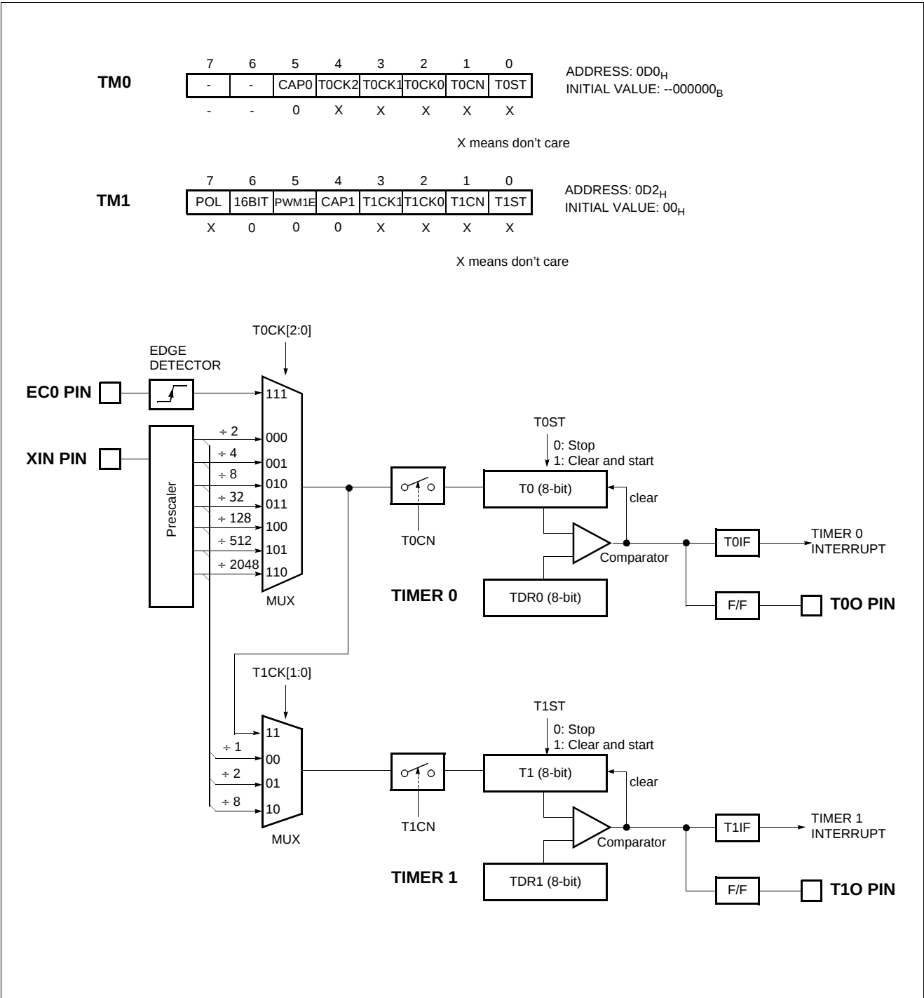
Figure 12-2 8-bit Timer/Counter 0, 1
