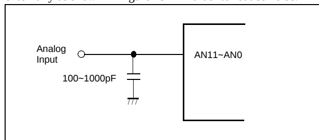
Figure 13-4 Analog Input Pin Connecting Capacitor
