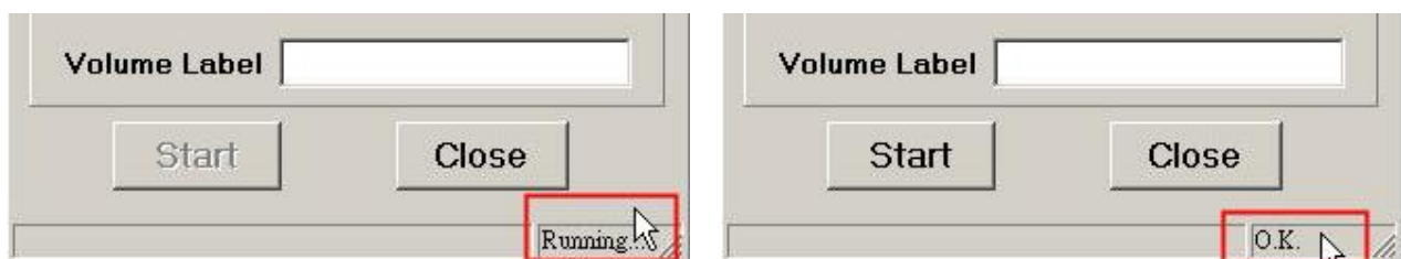
Figure 10: Format Complete
