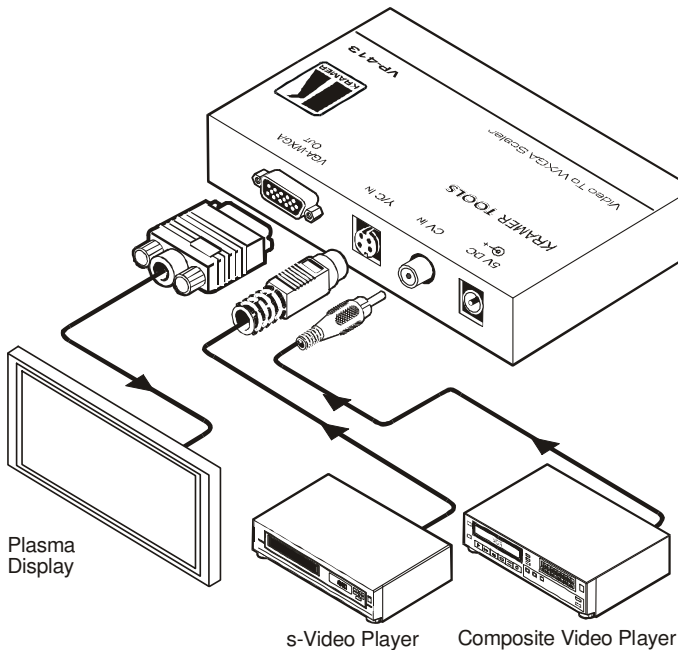
Figure 5: Connecting the VP-413
