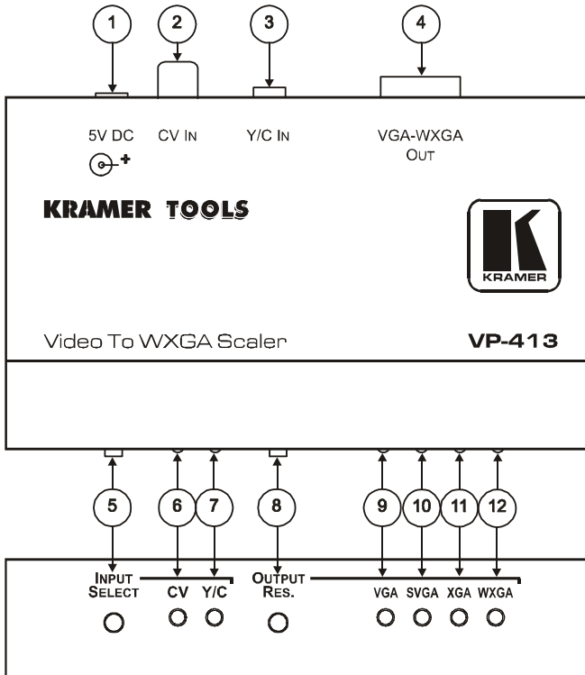
Figure 1: VP-413 Video to WXGA Scaler
