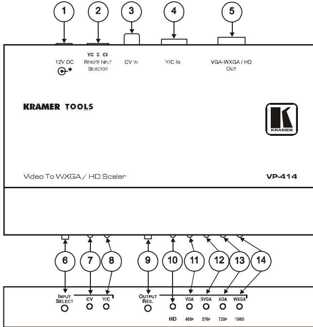
Figure 2: VP-414 Video to WXGA / HD Scaler
