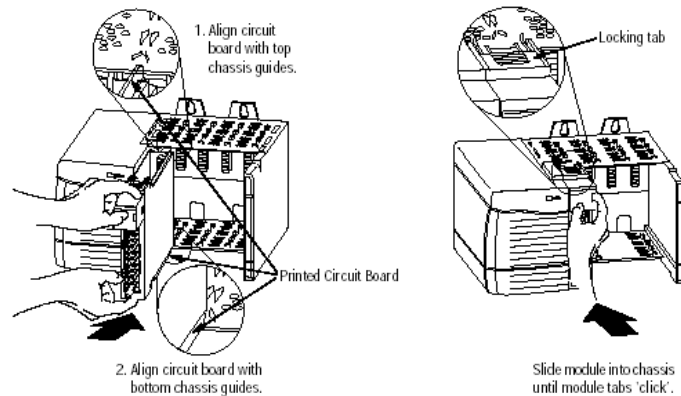
Figure 2.1. Module insertion into a rack
