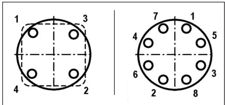
Figure 2-1 Torque Patterns
