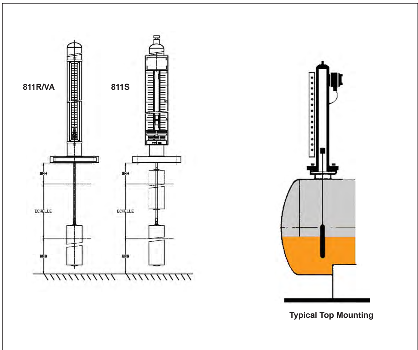
Figure 1-4 Top Mounting
