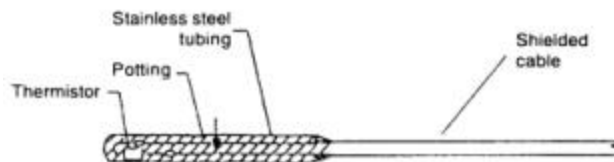
Figure 8, Thermistor sensor
