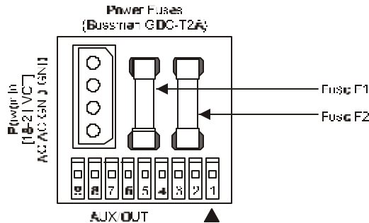
Figure 17, MCB Power Supply Terminals
