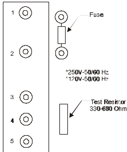
Figure 18, Output Board Relay Socket
