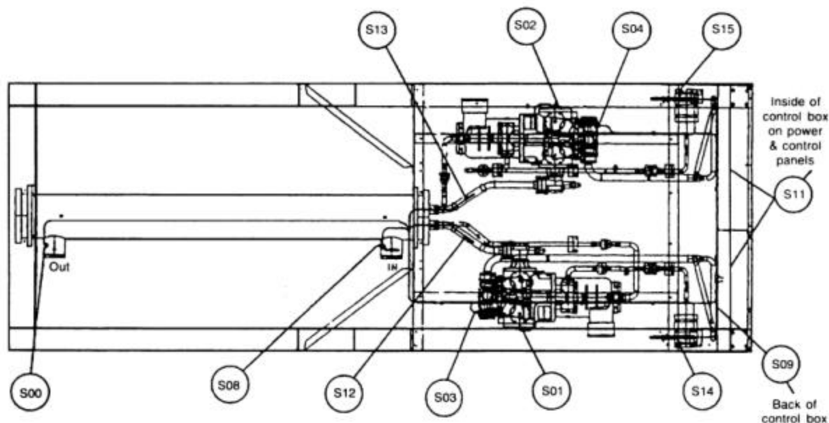
Figure 11, Sensor Locations, Two Compressor Units
