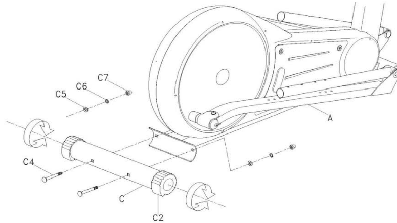
FIGURE 1 ASSEMBLY FOR REAR STABILIZER
