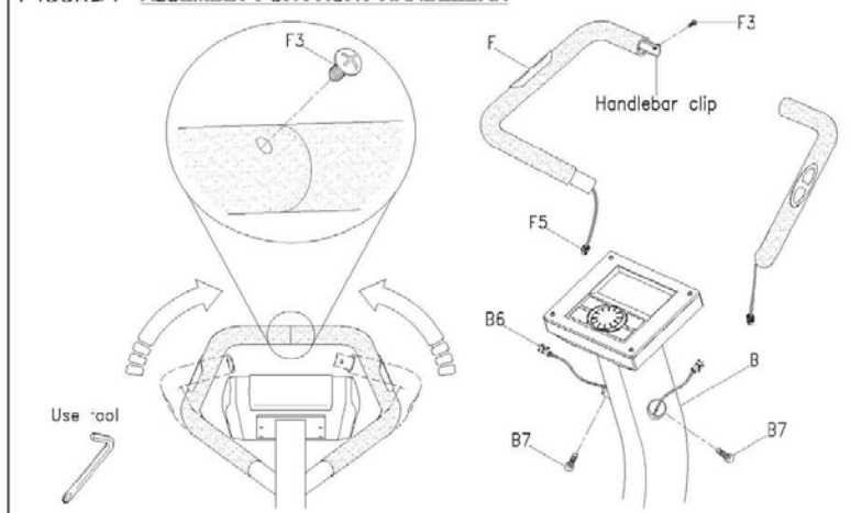
FIGURE 7 ASSEMBLY FOR FRONT HANDLEBAR
