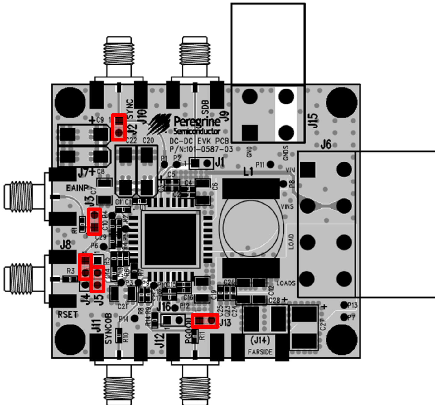
Figure 2. Evaluation Board Assembly
