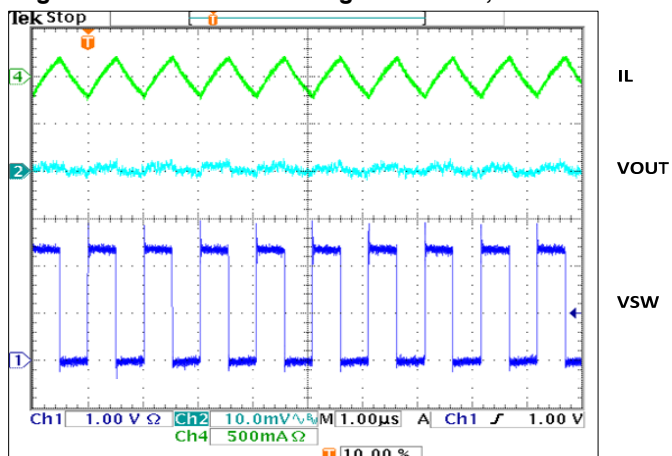
Figure 16. PE99155 Switching waveforms, 1 MHz
