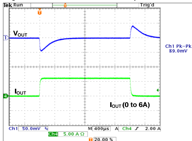
Figure 10. PE99153 Load Transient Response
