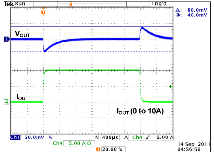
Figure 14. PE99155 Load Transient Response
