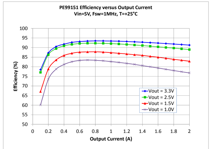
Figure 4. PE99151 Efficiency vs. Output Current
