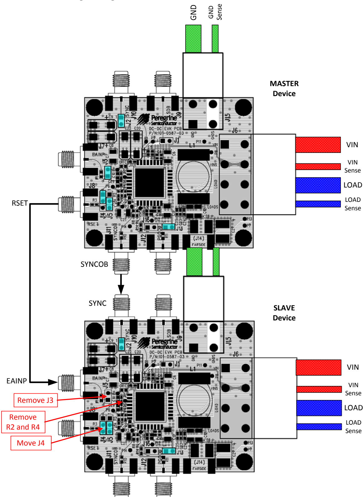
Figure 22. Current Sharing Configuration
