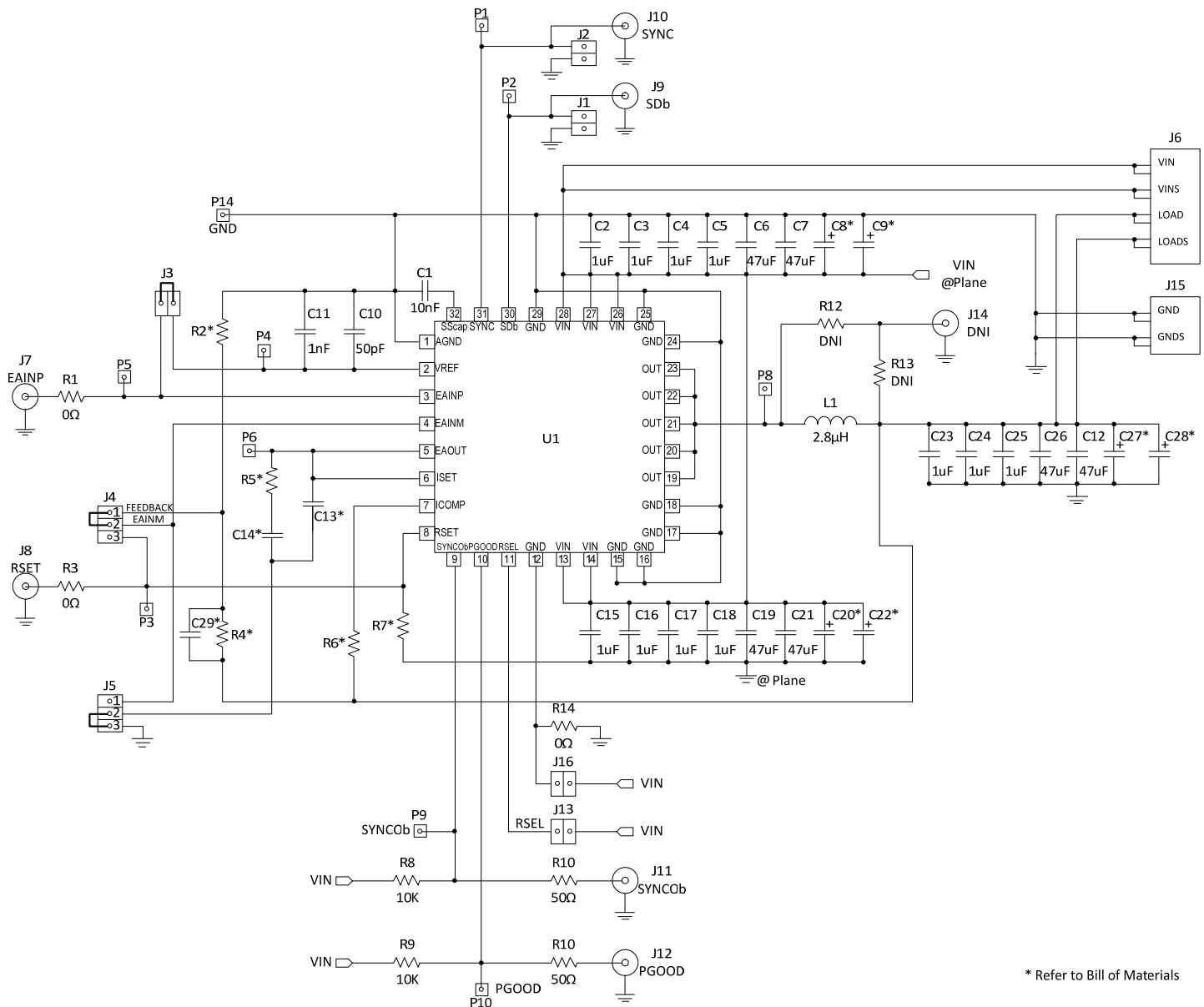
Figure 1. Evaluation Board Schematic
