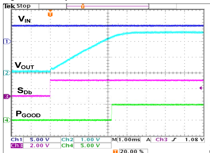
Figure 17. Start-up waveforms
