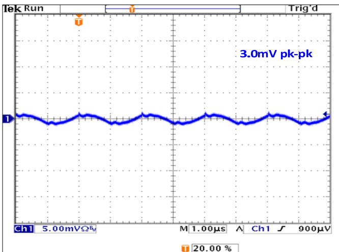
Figure 5. PE99151 Output Ripple
