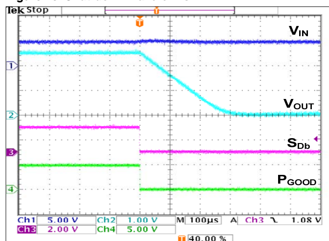
Figure 18. Shut-down waveforms
