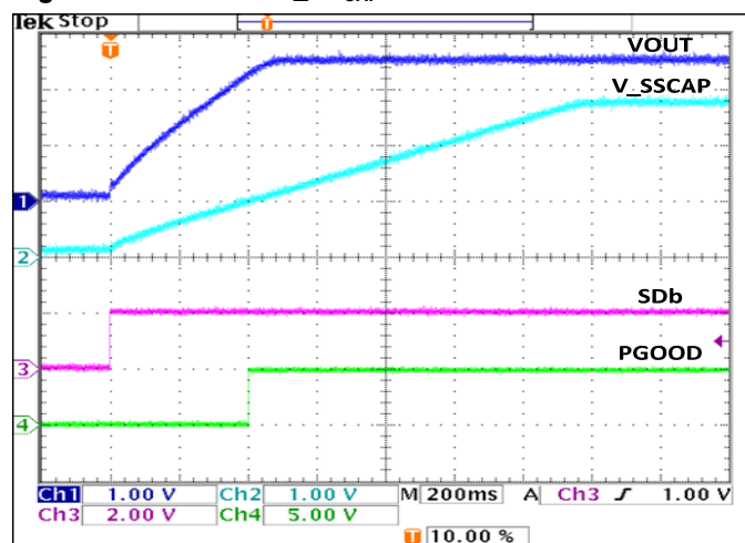
Figure 20. Soft Start C_{SSCAP} = 1000\text{ nF}
