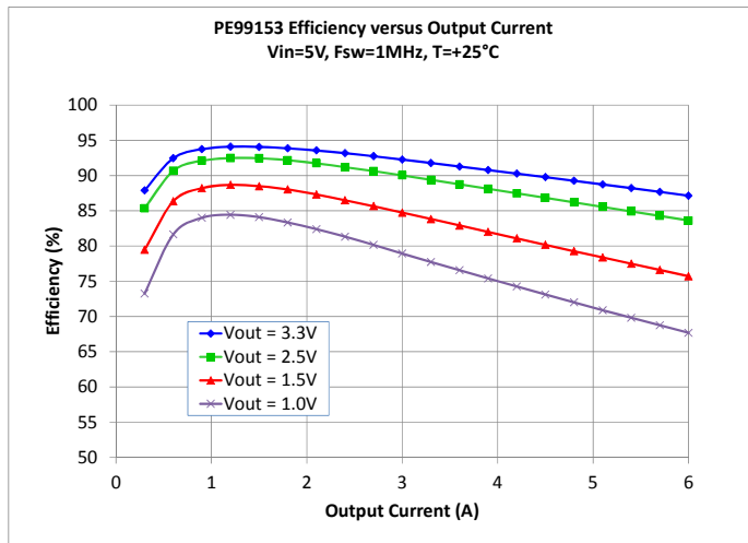
Figure 8. PE99153 Efficiency vs. Output Current
