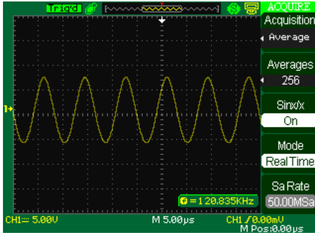
Figure 42 - Acquisition Averaging Screen
