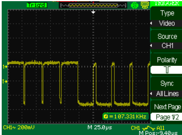
Figure 34 - Video Trigger Screen
