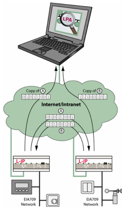
Figure 5: EIA852 Packet Logging
