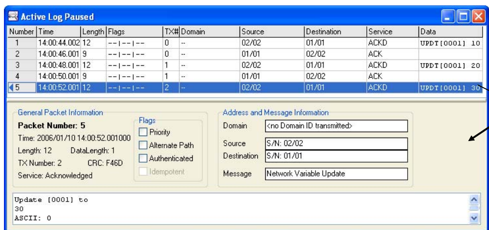
Figure 20: Packet Details
