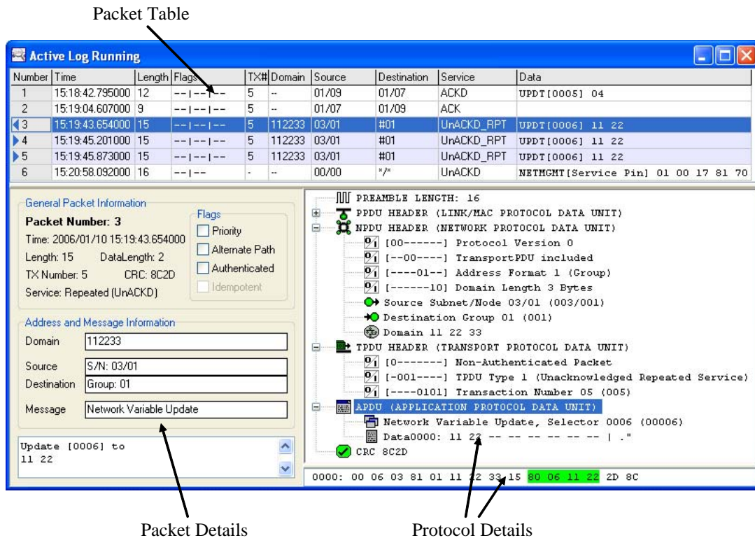
Figure 27: Log Window
