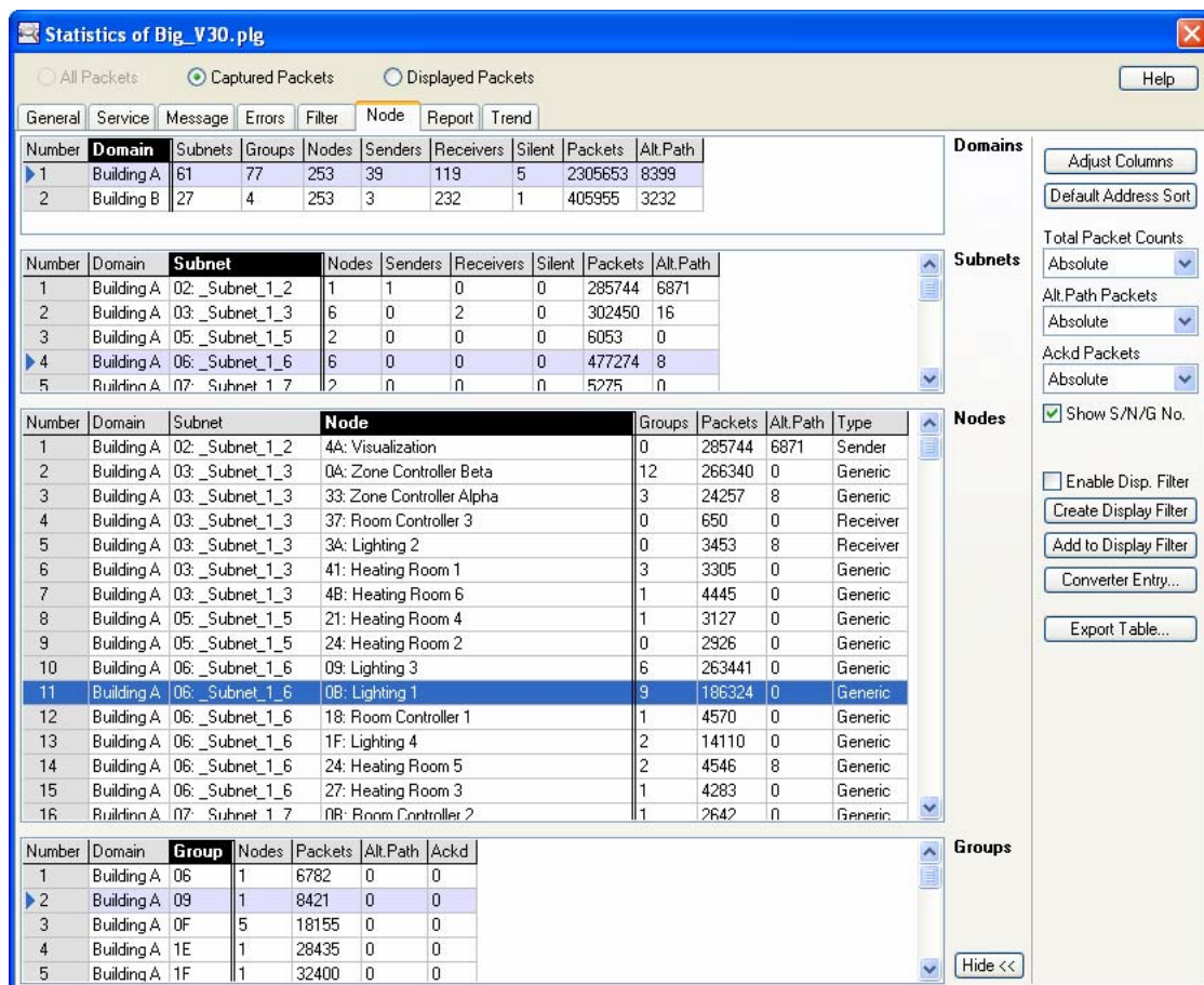
Figure 43: Node Statistics
