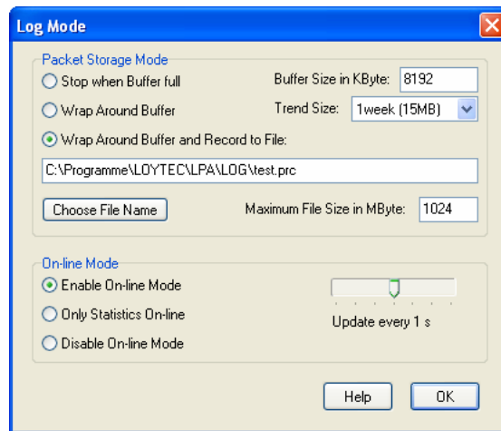
Figure 35: Log Mode
