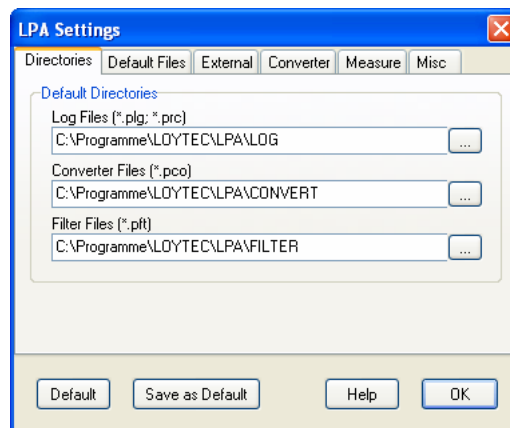
Figure 49: LPA Settings
