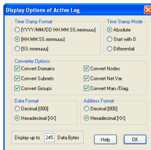
Figure 41: Display Options
