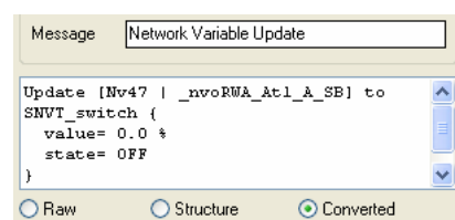
Figure 29: SNVT Messages
