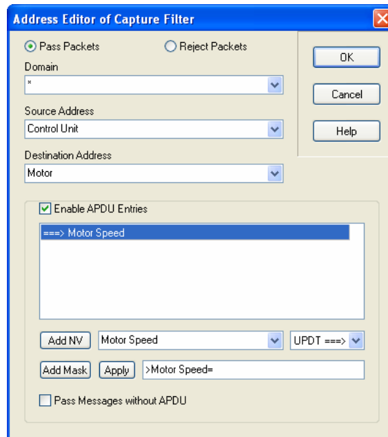
Figure 40: Address Editor
