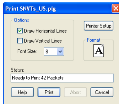
Figure 34: Print Log
