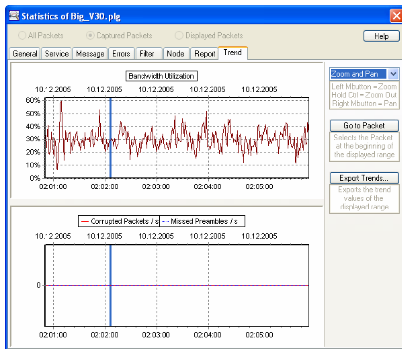
Figure 46: Statistics Trends
