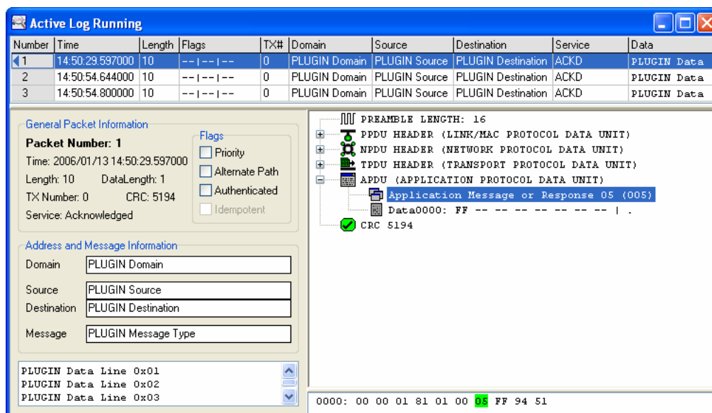
Figure 50: LPA Plug-In
