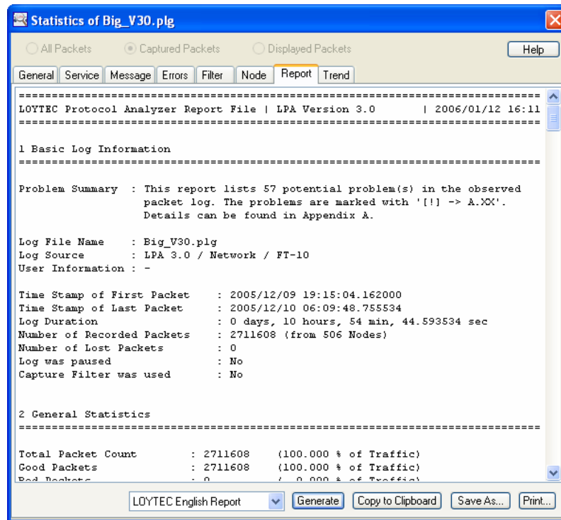
Figure 45: LPA Report
