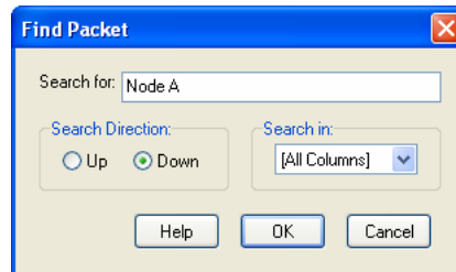
Figure 31: Find Packet
