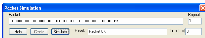
Figure 47: Packet Simulation
