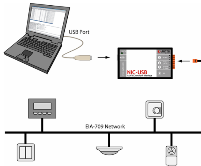
Figure 2: NIC709 Setup
