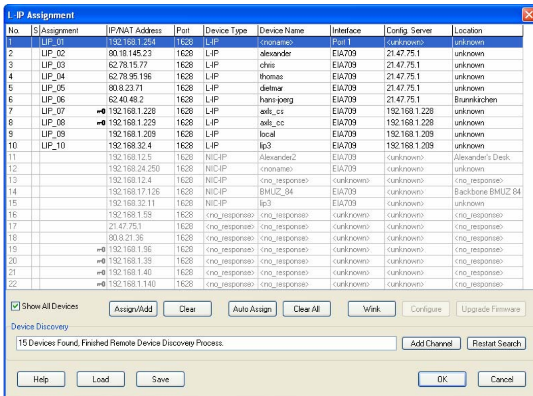
Figure 8: L-IP Assignment
