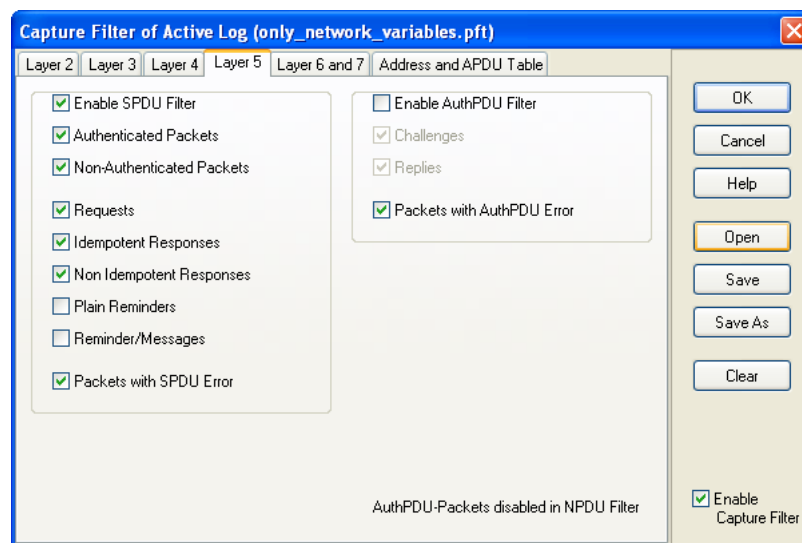
Figure 38: Packet Filter
