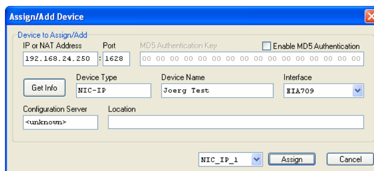
Figure 13: Assign/Add NIC-IP
