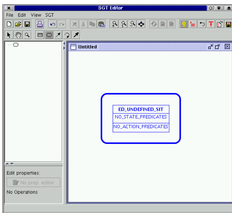
Figure 3.2: SGTEDITOR with one situation scheme and one situation graph.
