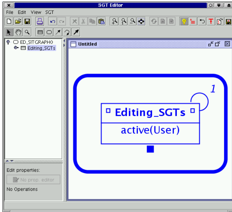
Figure 3.14: Semantic zooming: action predicates were hidden. In addition, the hidden specializing graph is indicated by a filled rectangle below the situation.
