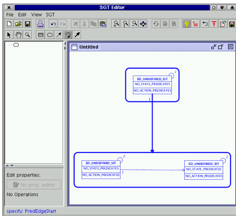
Figure 3.8: The resulting SGT after reactivation of Intelligent Mode , centering and maximization.
