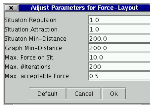
Figure 2.3: The dialog for adjusting all parameters of the force layout algorithm.
