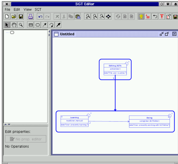
Figure 3.11: The resulting SGT after all three situation schemes have been edited.
