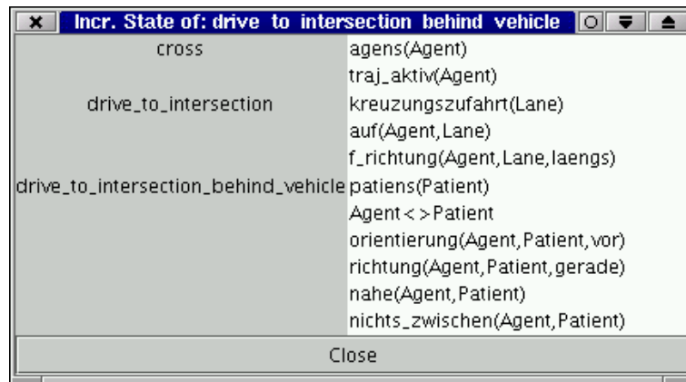
Figure 2.7: The dialog showing the incremental state scheme of one situation scheme.
