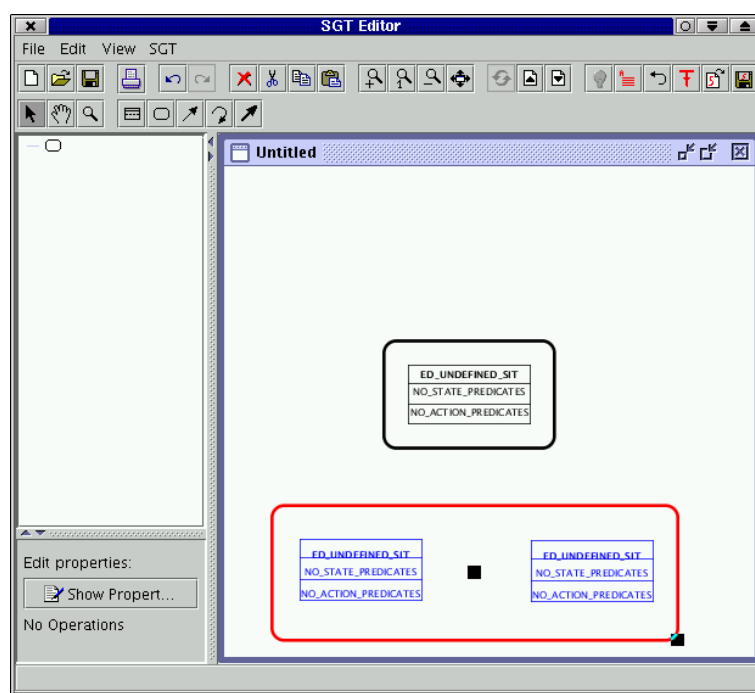
Figure 3.5: SGTEDITOR decides to declare lower graph as SGT.
