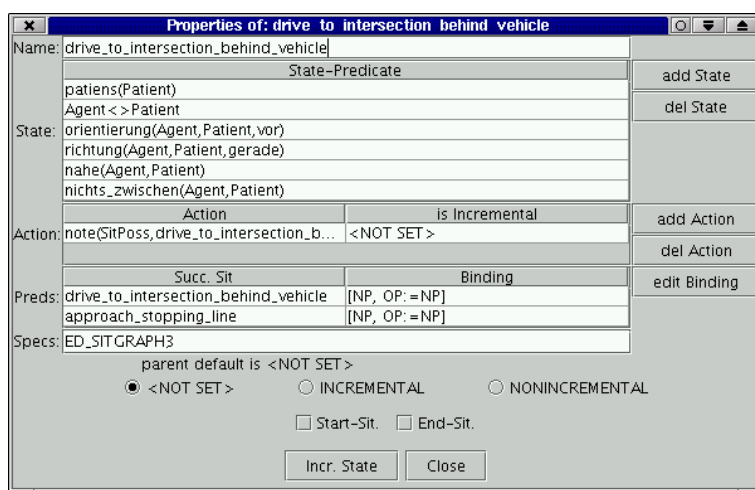
Figure 2.5: The property editor for situation schemes.
