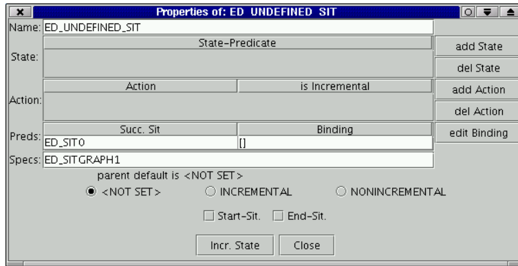
Figure 3.9: The property editor for the top-most situation scheme.
