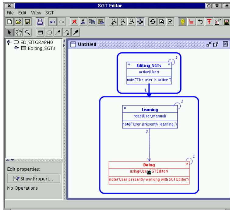
Figure 3.16: Layout after dragging one situation and thereby stacking the lower two situation schemes one on top of the other.
