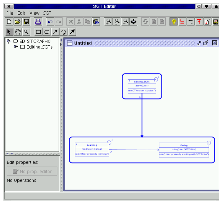
Figure 3.12: The tree view of the SGT was created and is depicted in the tree view panel (top-left of frame).
