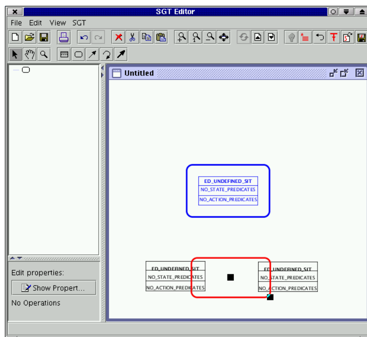
Figure 3.4: To resize a graph, select it and move the handle in the lower right corner.
