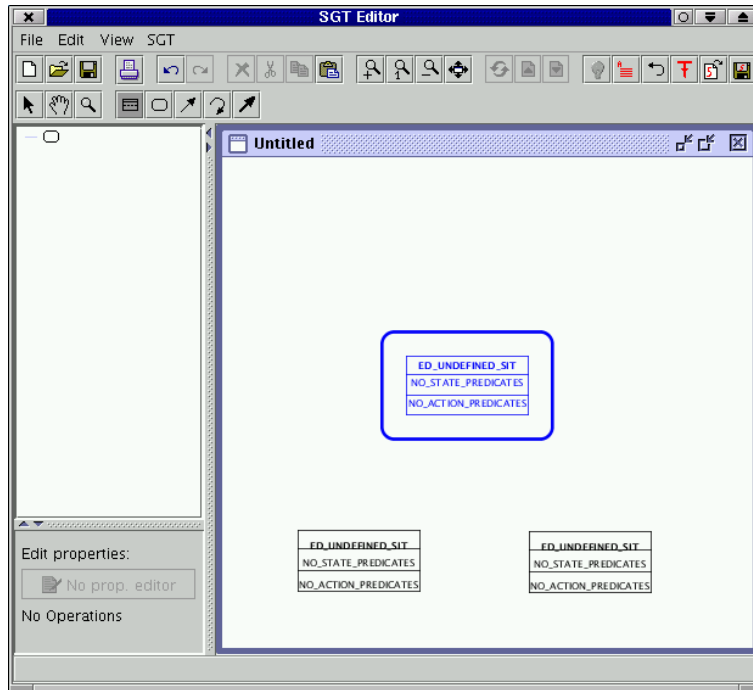
Figure 3.3: Some more situation schemes added.
