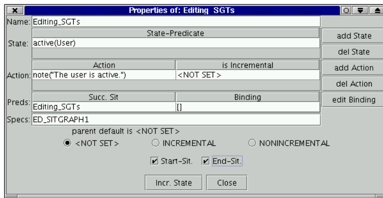
Figure 3.10: The same property editor as before with some entries changed.
