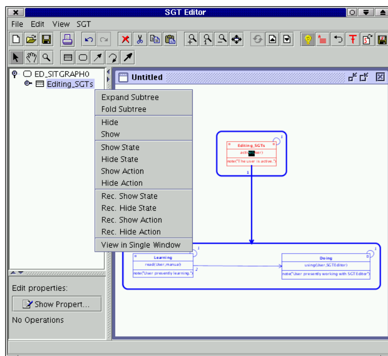
Figure 3.13: The tree view with opened context-menu.
