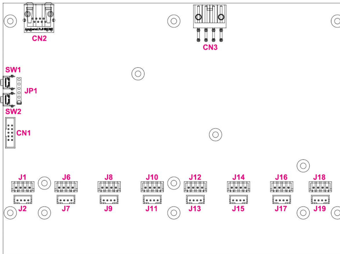
Bottom View
