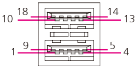
Connector pin definition
