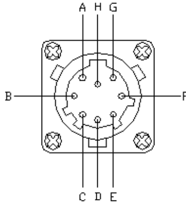
Figure A.2.1-2 LAN connector
