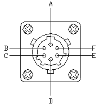
Figure A.1.1-3 Keyboard connector
