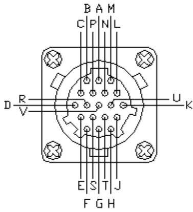
Figure A.1.1-1 USB1 Connector
