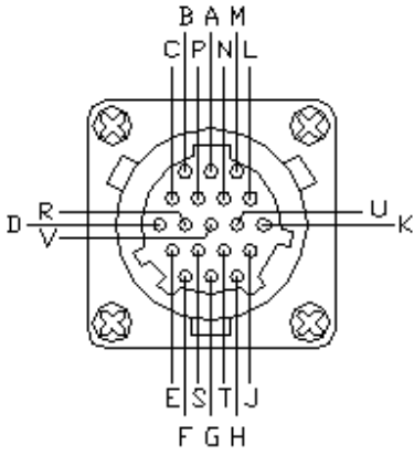
Figure A.2.1-1 USB1 Connector
