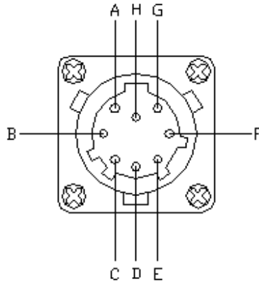
Figure A.1.1-2 LAN connector
