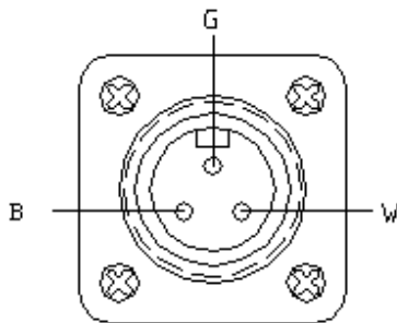
Figure A.1.1-4 AC power input Connector
