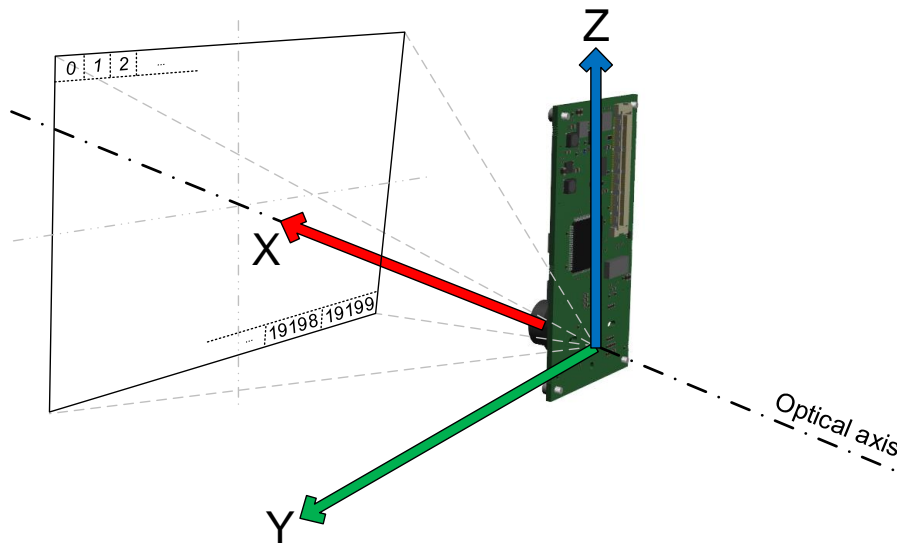
Figure 4-2: TIM-UP-19K-S3-ETH Default Coordinate System
