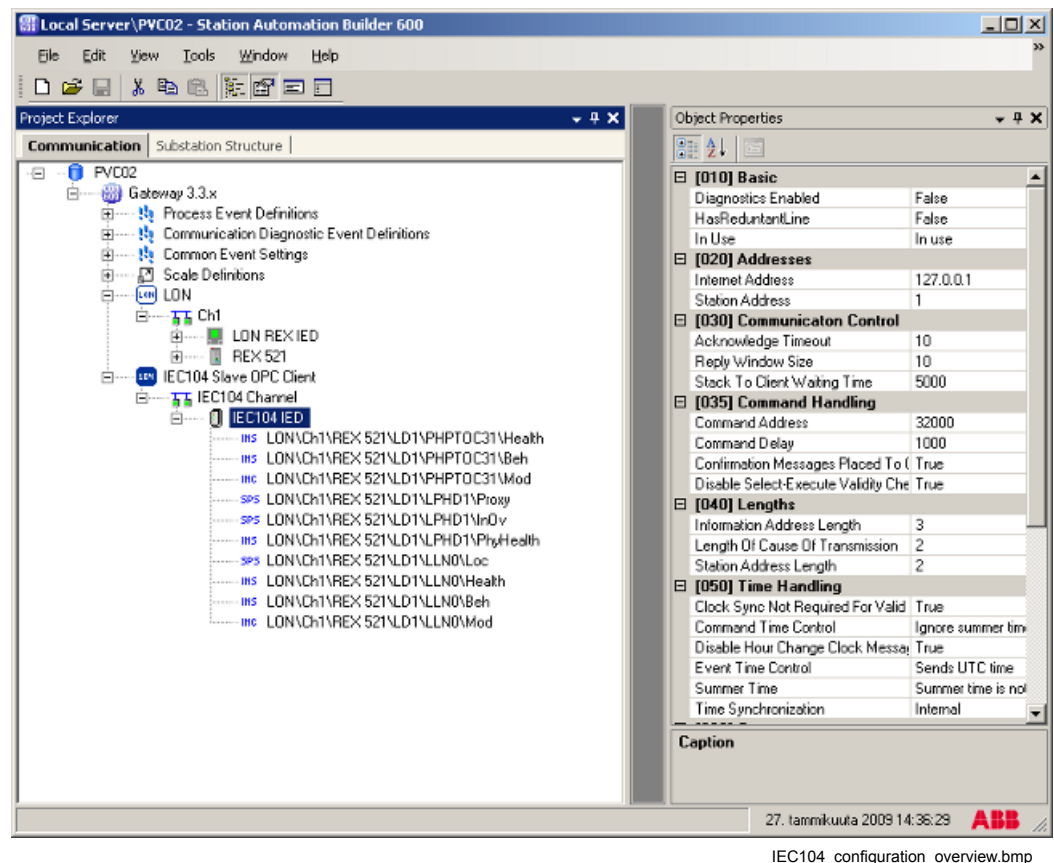
Figure 3.2-1 Example view of SAB600
