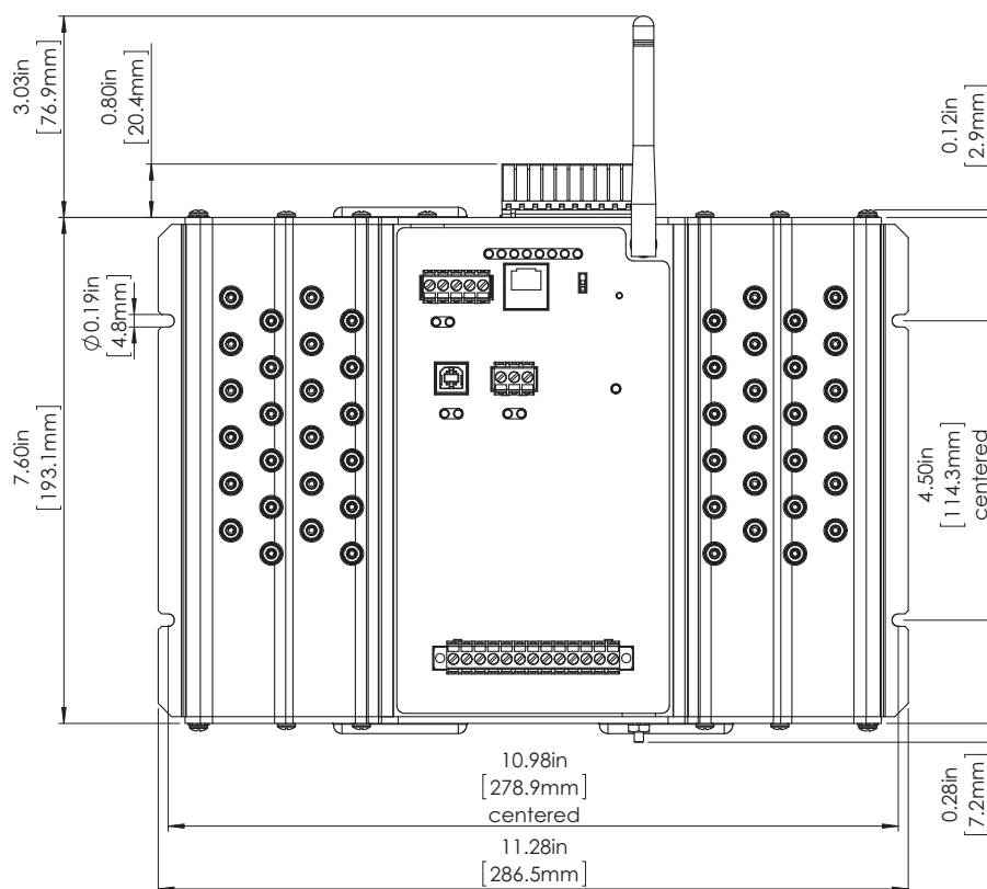
FIGURE 3.1: EPM 4600 Unit Front Dimensions
