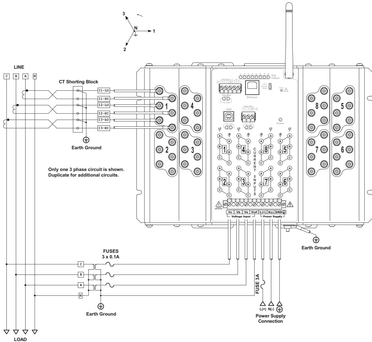
FIGURE 4.6: Three Phase, 4-Wire WYE Service with 3 PT Voltage and 3 CT Connection for Metering 8 Three Phase Loads: EPM 4600-T
