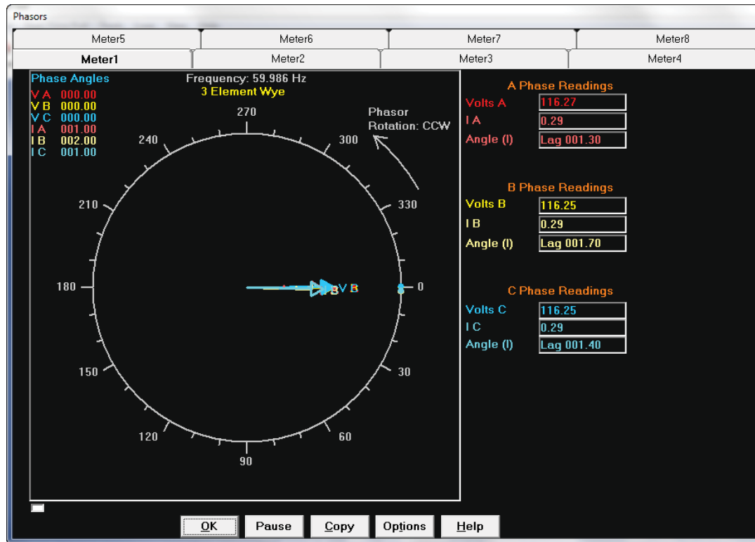
Three Phase Configuration
