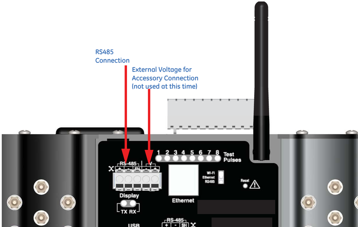
FIGURE 5.6: FCom 3 RS485 Port
