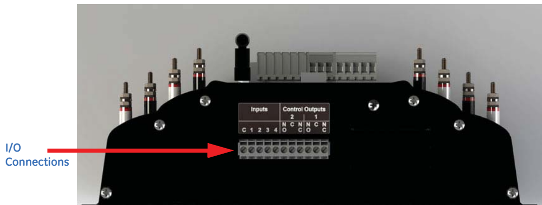
FIGURE 7.1: Location of I/O Board
