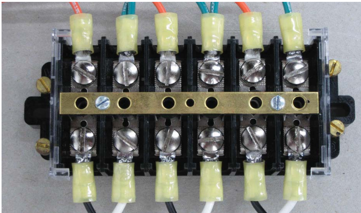
FIGURE 4.10: Typical Shorting Block with Wiring Installed
