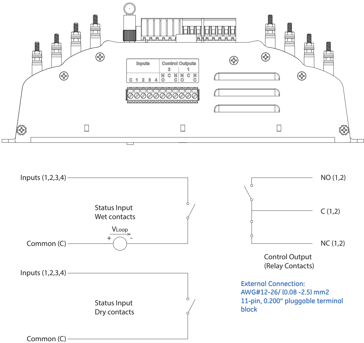
FIGURE 7.2: Relay Contact (4) / Status Input (2) I/O Wiring
