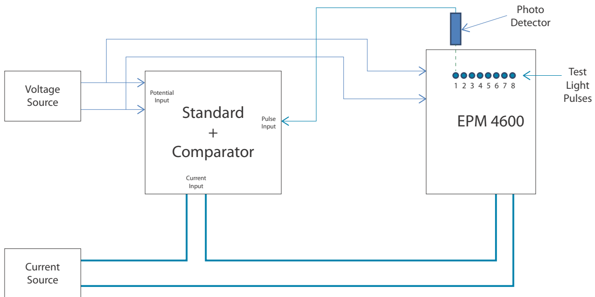
FIGURE 6.3: Typical Kh Test Setup
