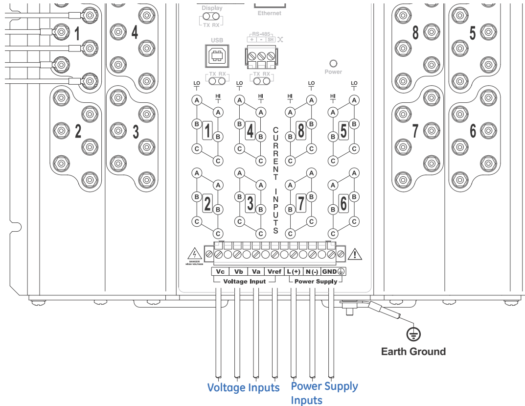
FIGURE 4.2: EPM 4600 Unit Connections
