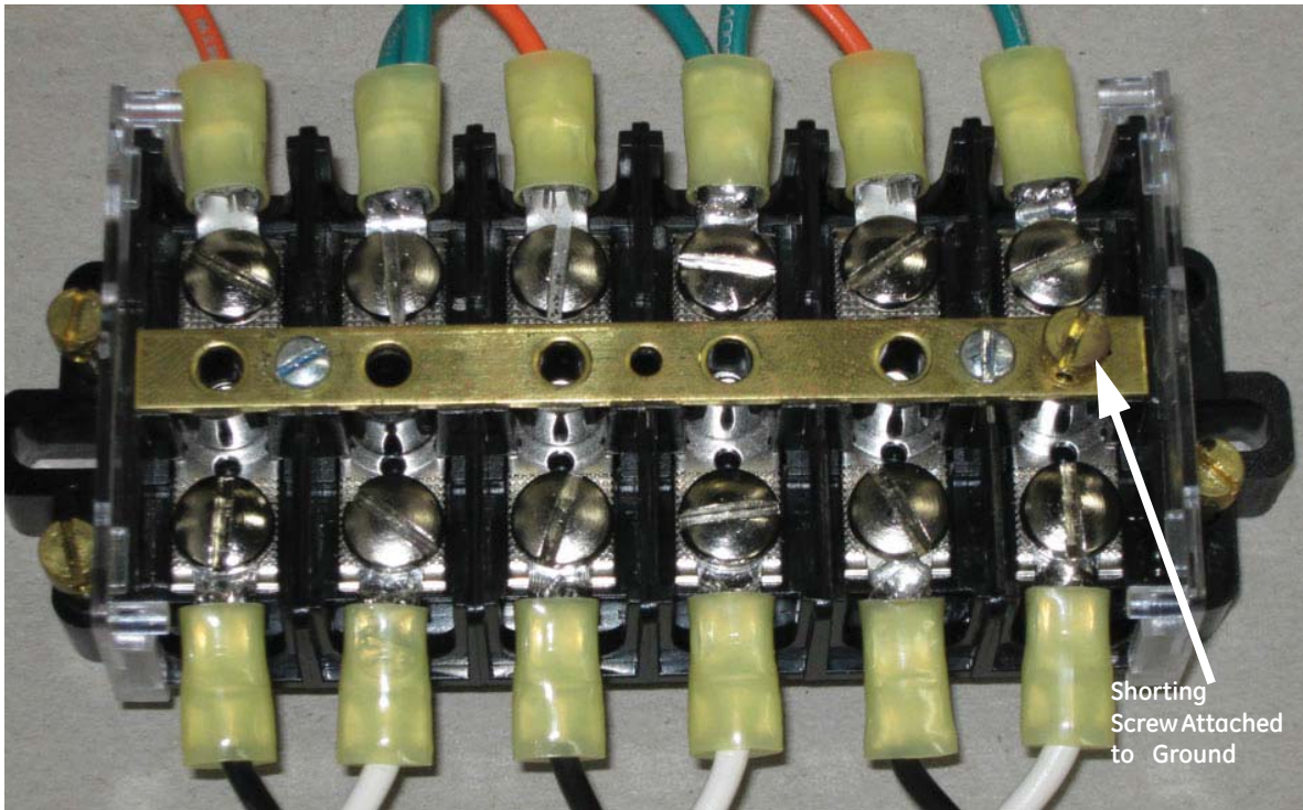
FIGURE 4.11: Shorting Block with Shorting Screw Attached to Ground Terminal
