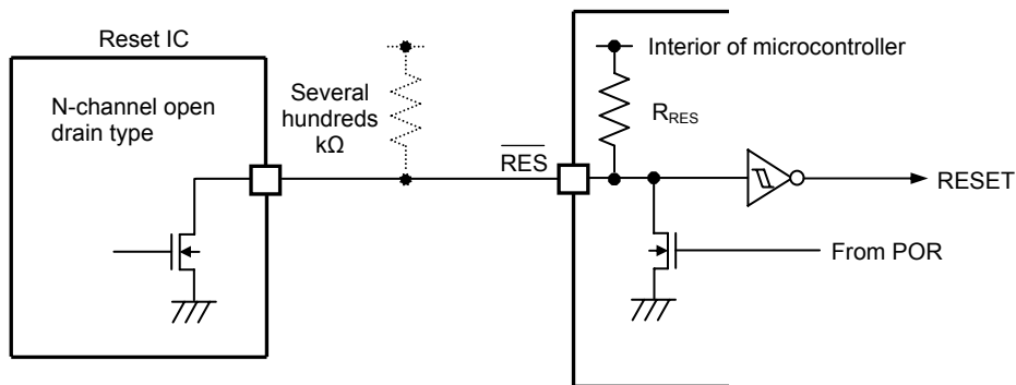
Figure 4.5.5 Sample Reset Circuit Configuration Using an N-channel Open Drain Type Reset IC
