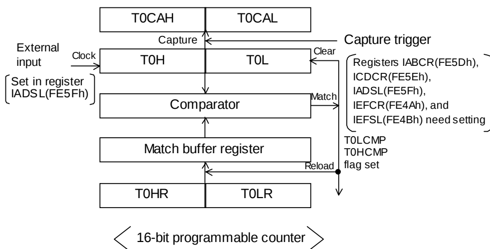
Figure 3.3.4 Mode 3 Block Diagram (T0LONG = 1, T0LEXT = 1)
