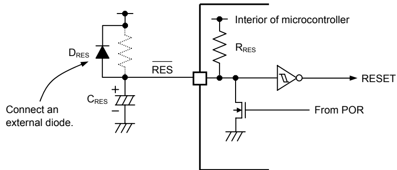
Figure 4.5.7 Sample External POR Circuit Configuration
