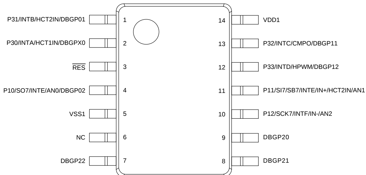
SANYO: MFP14S (for debugging only) (Lead-free type)
