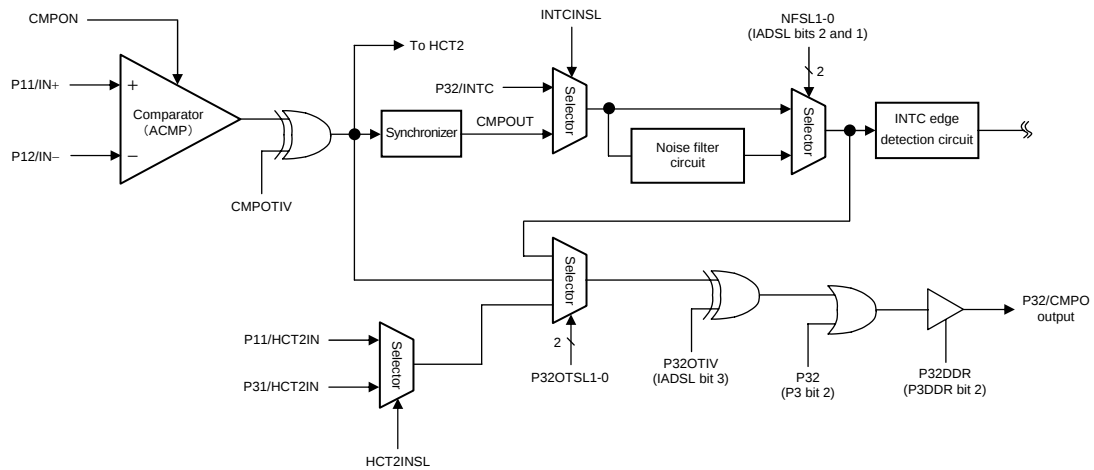
Figure 3.10.1 Analog Comparator and P32/CMPO Multiplexed Pin Output Block Diagram
