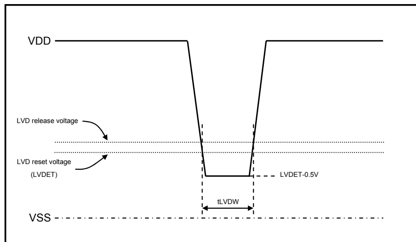
Figure 4.5.3 Example of Power Interruption or Voltage Fluctuation Waveform
