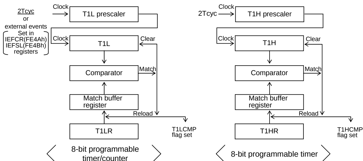
Figure 3.4.1 Mode 0 (T1LONG = 0) Block Diagram
