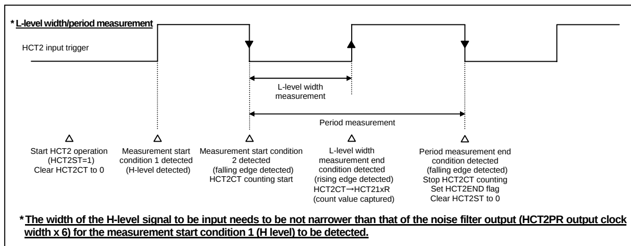
Figure 3.8.2 Sample High-speed Pulse Width /Period Measurement Counter 2 Waveforms
