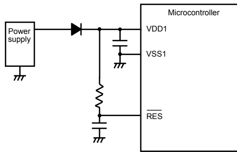
Figure 4.5.4 Example of Power Interruption / Voltage Fluctuation Countermeasures
