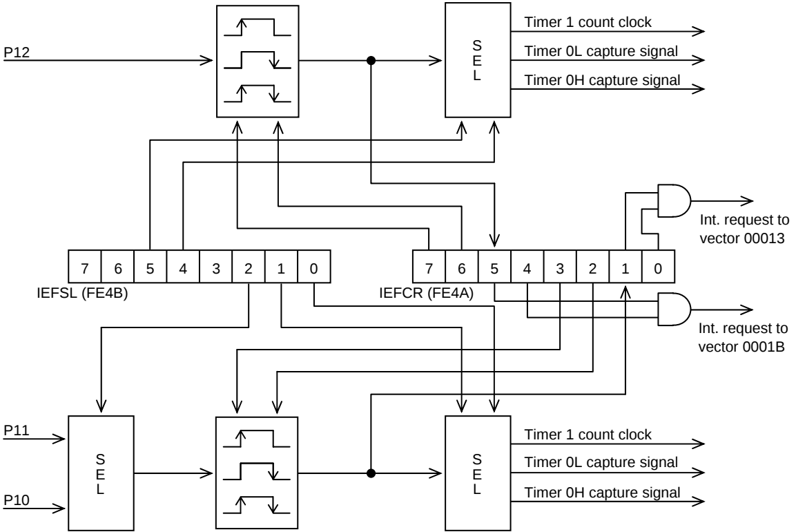
Port 1 (Interrupt) Block Diagram
