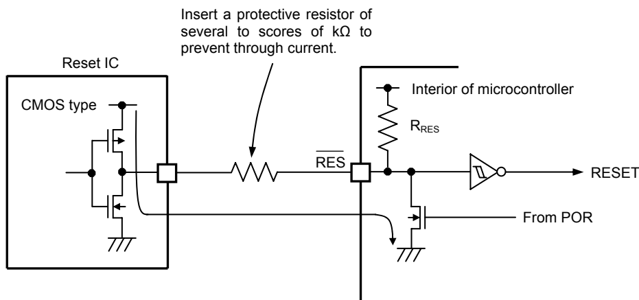
Figure 4.5.6 Sample Reset Circuit Configuration Using a CMOS Type Reset IC
