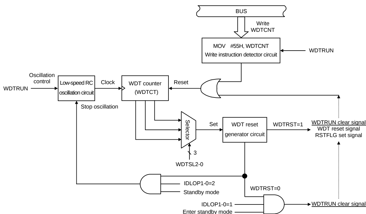
Figure 4.6.1 Watchdog Timer Operation Block Diagram
