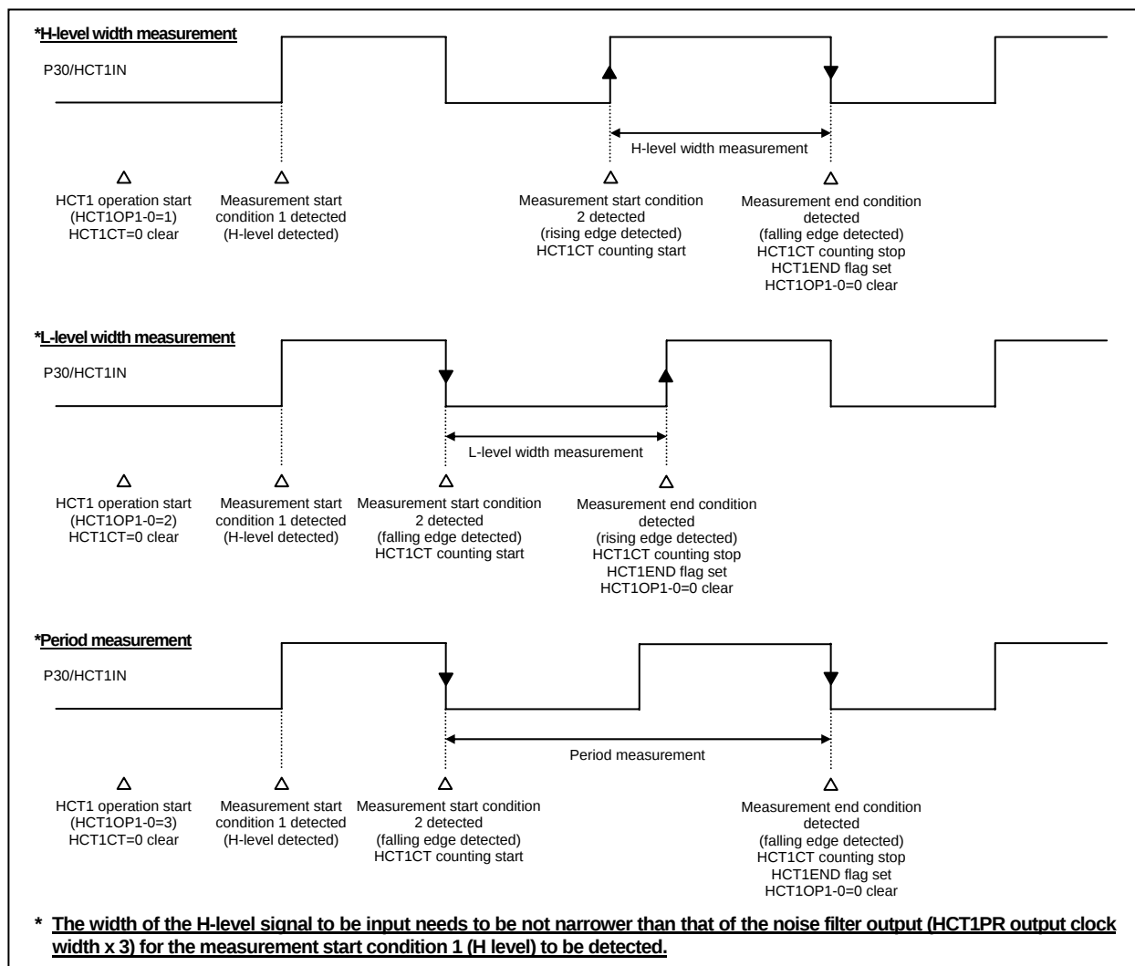
Figure 3.7.2 Sample High-speed Pulse Width/Period Measurement Counter 1 Waveforms
