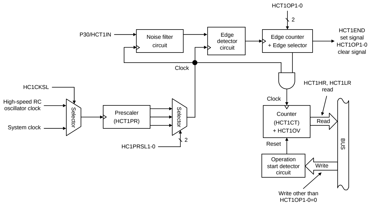
Figure 3.7.1 High-speed Pulse Width/Period Measurement Counter 1 Block Diagram
