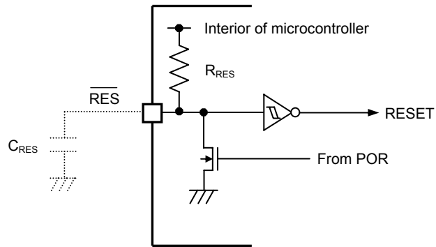
Figure 4.5.2 Reset Circuit Configuration Using only the internal POR Function
