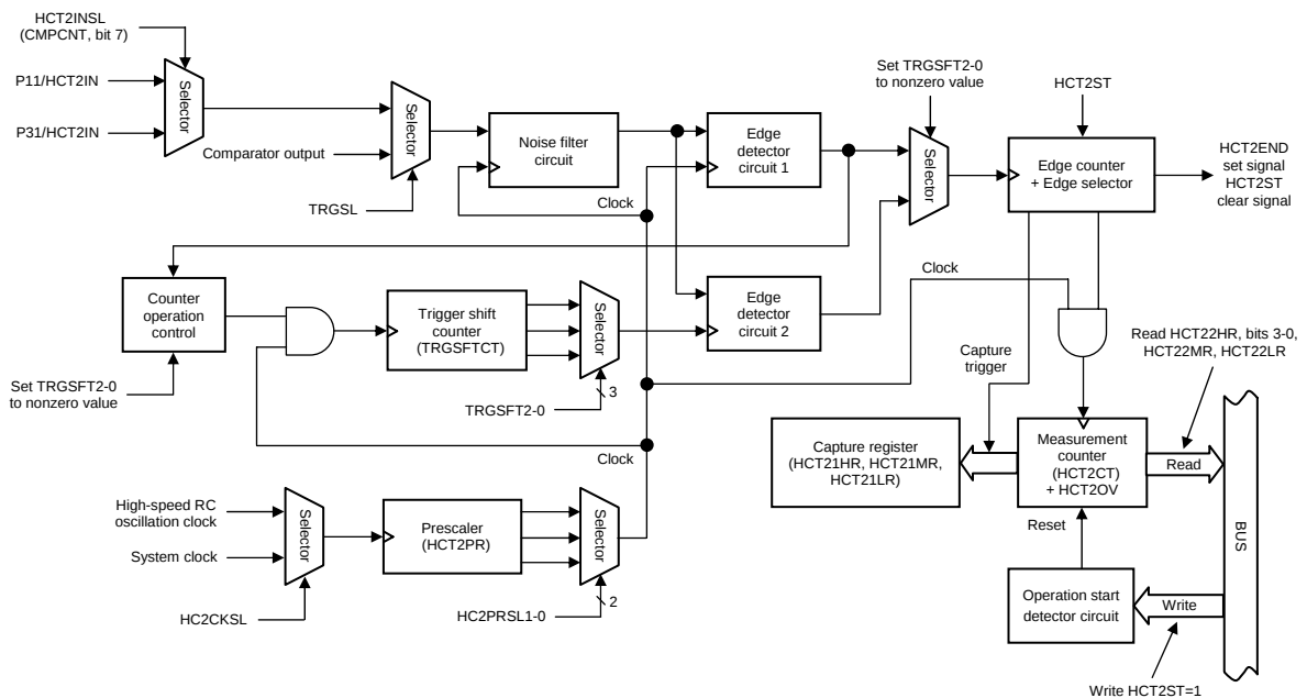
Figure 3.8.1 High-speed Pulse Width/Period Measurement Counter 2 Block Diagram
