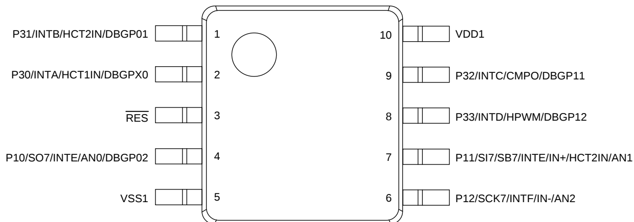
SANYO: MFP10S (Lead-/Halogen-free type)
