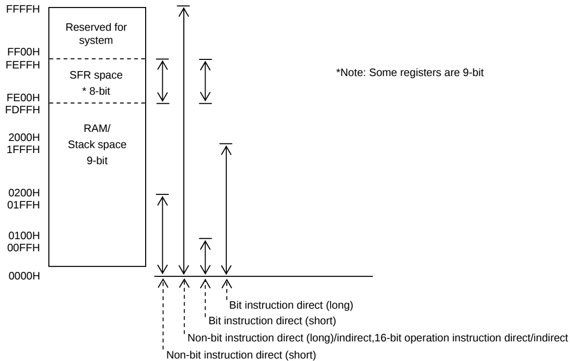
Fig. 2.4.1 RAM Addressing Map
