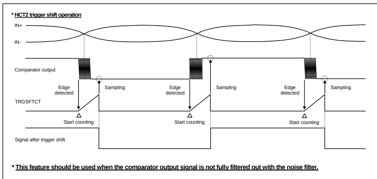
Figure 3.8.3 Sample Input Trigger Signal Shift Operation Waveforms (TRGSFT2 to TRGSFT0 set to a nonzero value)
