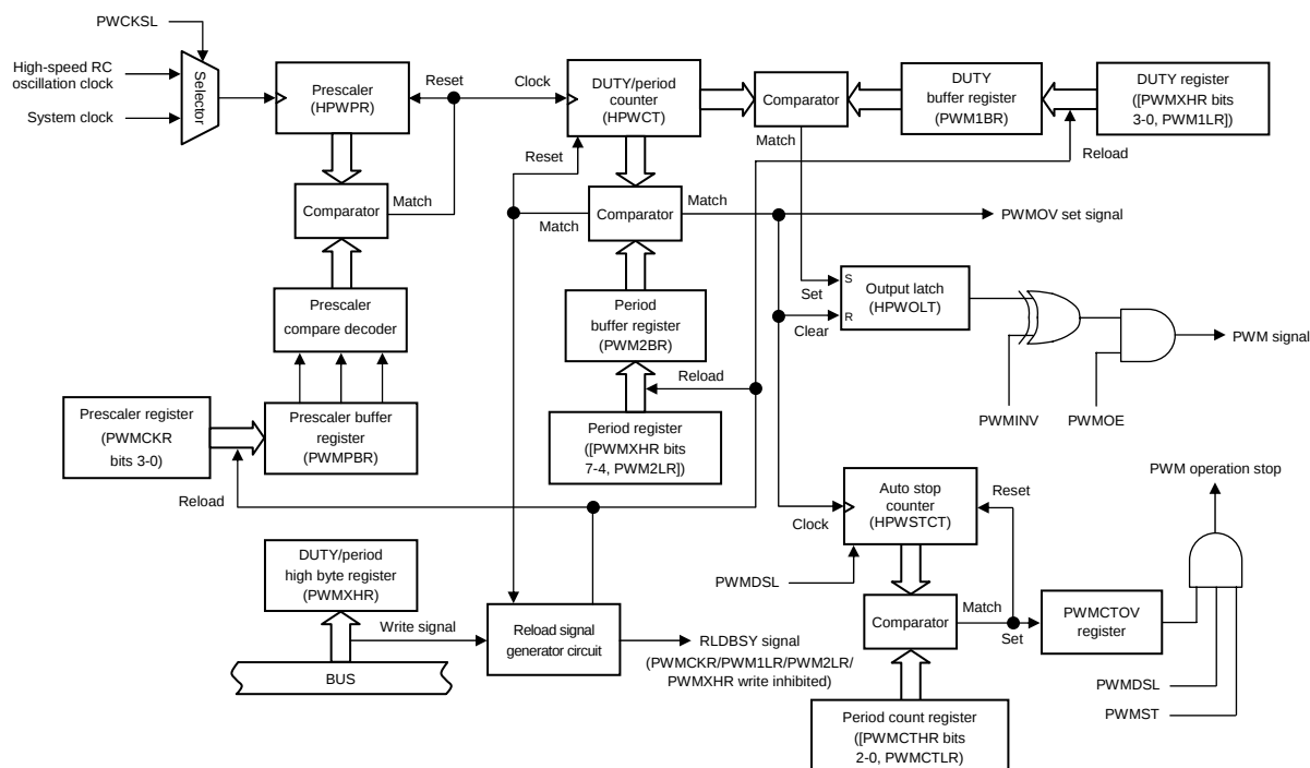
Figure 3.6.1 High-speed 12-bit PWM Block Diagram
