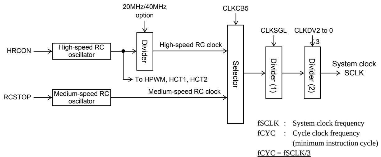
Figure 4.2.1 System Clock Generator Block Diagram
