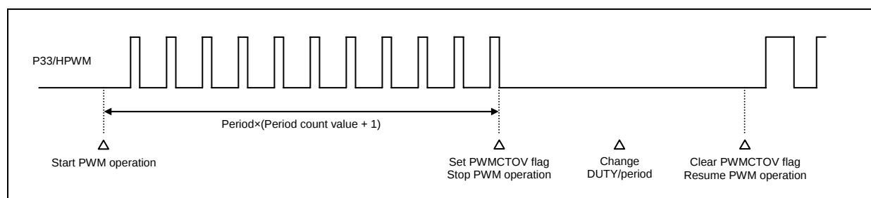
Figure 3.6.3 Sample Preset Value Output (Auto Stop) Mode Waveform (PWMINV=0)
