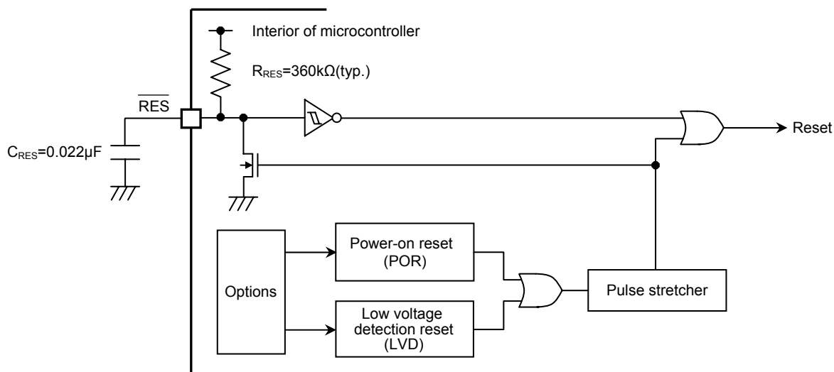
Figure 4.5.1 Internal Reset Circuit Configuration
