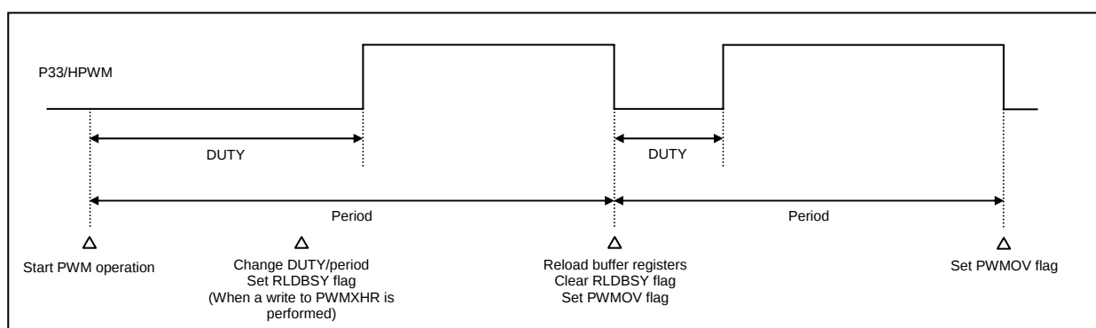
Figure 3.6.2 Sample Continuous Output Mode Waveform (PWMINV=0)
