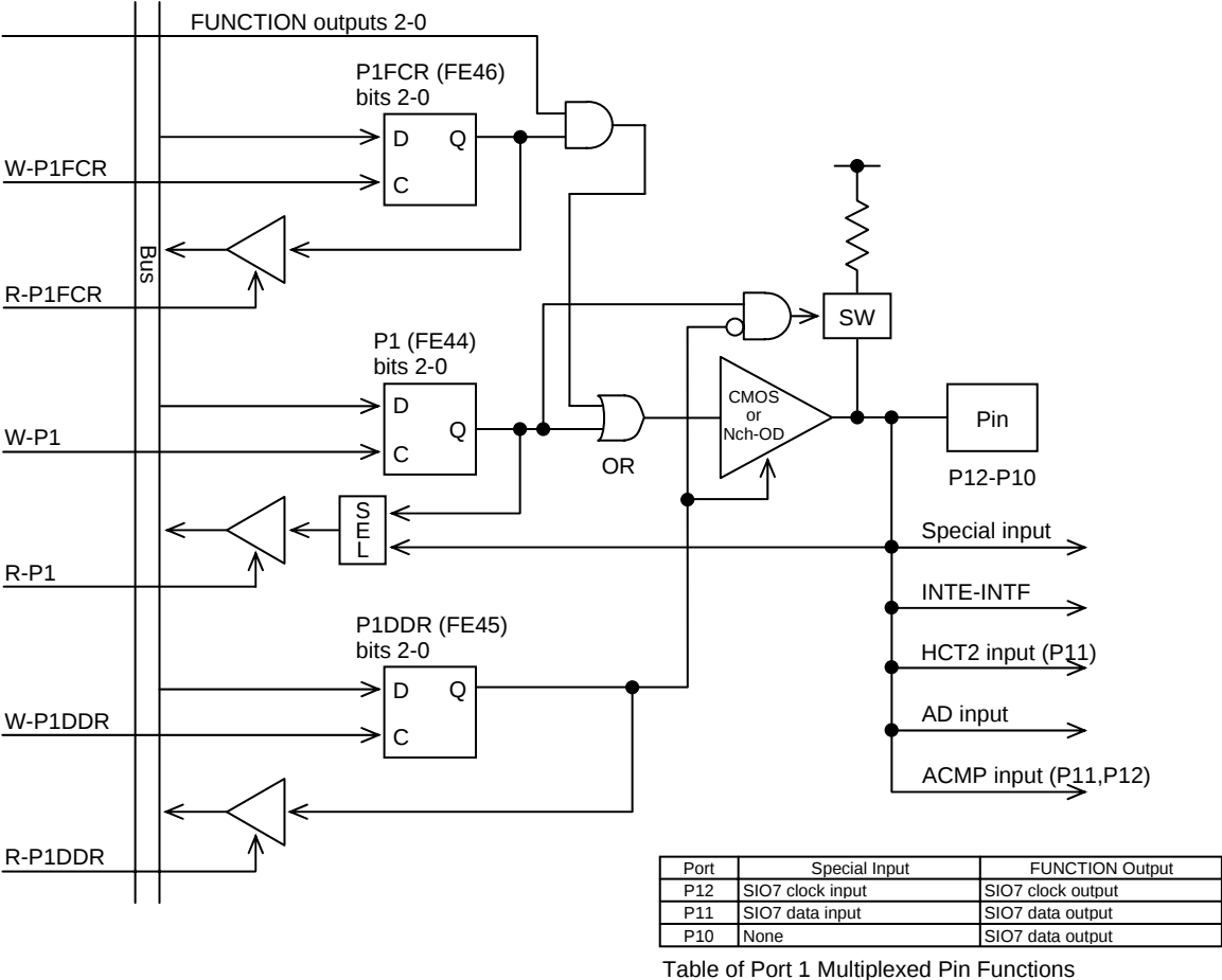
Port 1 Block Diagram (1) Option: Output type (CMOS or Nch-OD) selectable on a bit basis.
