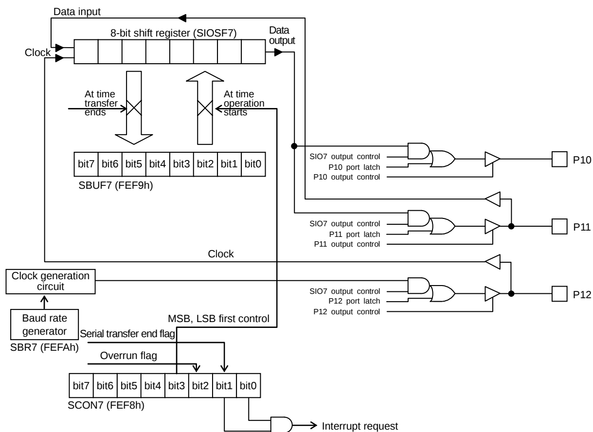
Figure 3.5.1 SIO7 Synchronous 8-bit Serial I/O Block Diagram
