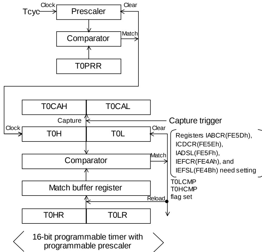
Figure 3.3.3 Mode 2 Block Diagram (T0LONG = 1, T0LEXT = 0)
