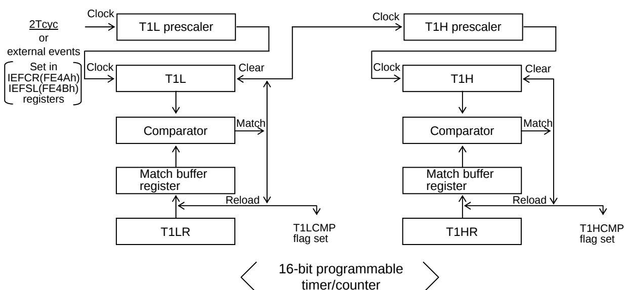
Figure 3.4.2 Mode 2 (T1LONG = 1) Block Diagram
