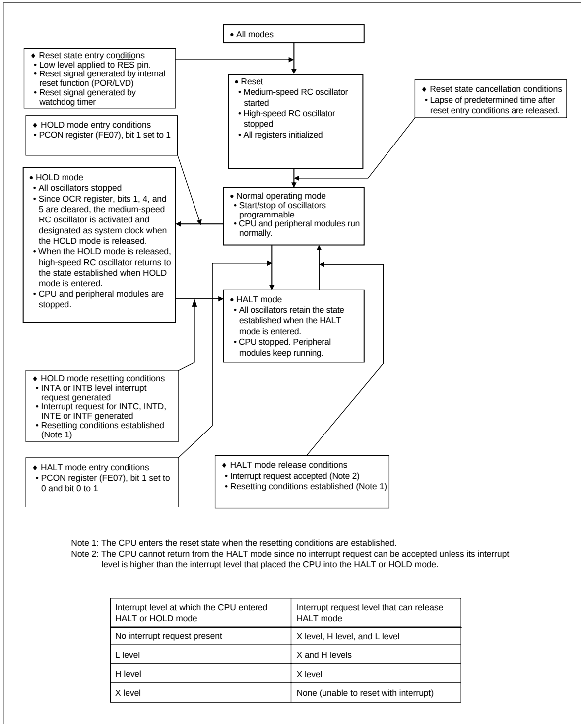
Figure 4.3.1 Standby Mode State Transition Diagram
